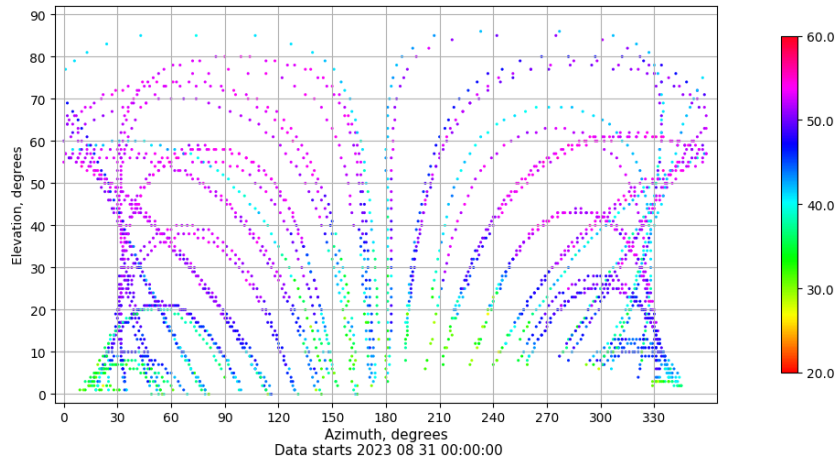
Azimuth-elevation plot for station EIVI. Signal to Noise S1C Data file EIVI00ESP_R_2023243.xtr
