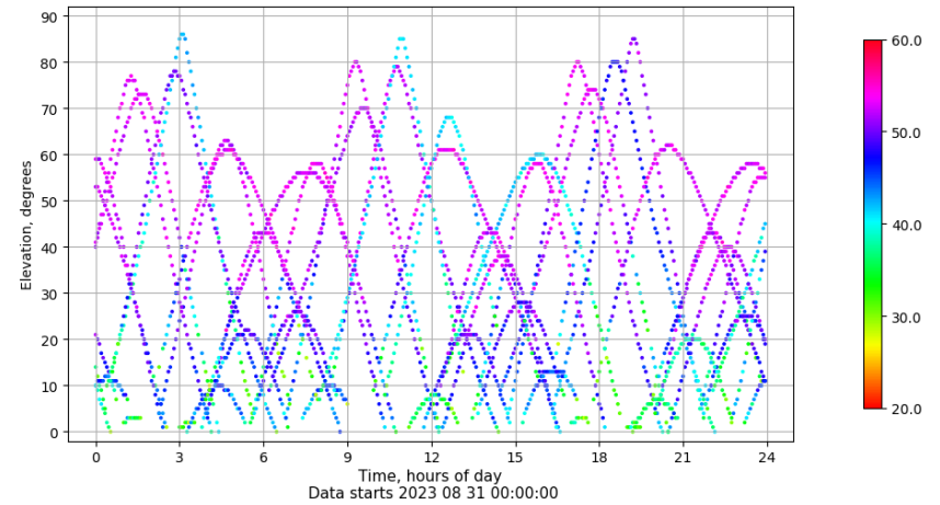
Time-elevation plot for station EIVI. Signal to Noise S1C Data file EIVI00ESP_R_2023243.xtr
