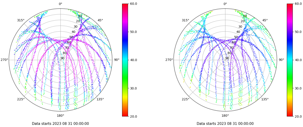
Skyplot for station EIVI. Signal to Noise S1C Data file EIVI00ESP_R_2023243.xtr Skyplot for station EIVI. Signal to Noise S2P Data file EIVI00ESP_R_2023243.xtr
