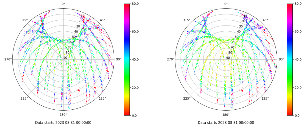
Skyplot for station EIVI. Parameter M1C Data file EIVI00ESP_R_2023243.xtr Skyplot for station EIVI. Parameter M2P Data file EIVI00ESP_R_2023243.xtr
