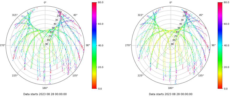
Skyplot for station EIVI. Parameter M1C Data file EIVI00ESP_R_2023240.xtr Skyplot for station EIVI. Parameter M2P Data file EIVI00ESP_R_2023240.xtr
