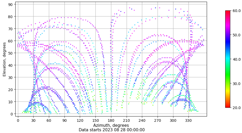
Azimuth-elevation plot for station EIVI. Signal to Noise S1C Data file EIVI00ESP_R_2023240.xtr
