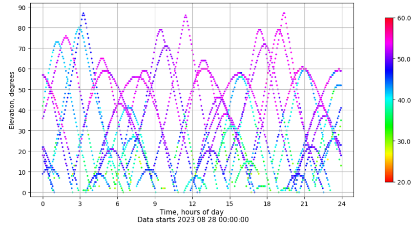
Time-elevation plot for station EIVI. Signal to Noise S1C Data file EIVI00ESP_R_2023240.xtr
