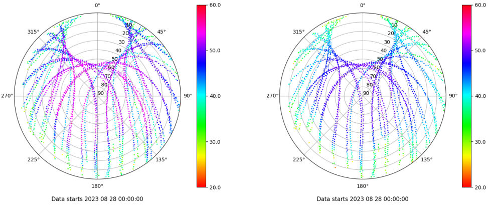
Skyplot for station EIVI. Signal to Noise S1C Data file EIVI00ESP_R_2023240.xtr Skyplot for station EIVI. Signal to Noise S2P Data file EIVI00ESP_R_2023240.xtr
