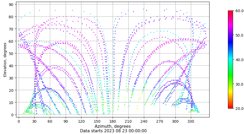
Azimuth-elevation plot for station EIVI. Signal to Noise S1C Data file EIVI00ESP_R_2023235.xtr
