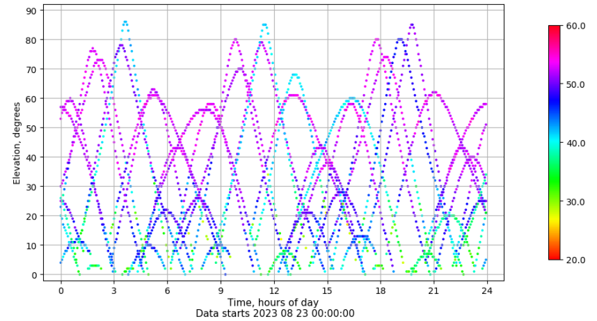
Time-elevation plot for station EIVI. Signal to Noise S1C Data file EIVI00ESP_R_2023235.xtr
