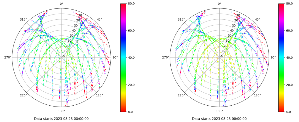
Skyplot for station EIVI. Parameter M1C Data file EIVI00ESP_R_2023235.xtr Skyplot for station EIVI. Parameter M2P Data file EIVI00ESP_R_2023235.xtr
