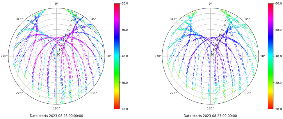
Skyplot for station EIVI. Signal to Noise S1C Data file EIVI00ESP_R_2023235.xtr Skyplot for station EIVI. Signal to Noise S2P Data file EIVI00ESP_R_2023235.xtr
