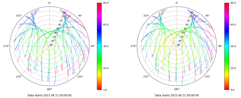
Skyplot for station EIVI. Parameter M1C Data file EIVI00ESP_R_2023233.xtr Skyplot for station EIVI. Parameter M2P Data file EIVI00ESP_R_2023233.xtr
