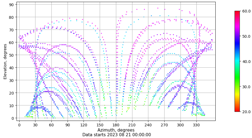
Azimuth-elevation plot for station EIVI. Signal to Noise S1C Data file EIVI00ESP_R_2023233.xtr
