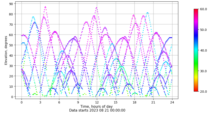
Time-elevation plot for station EIVI. Signal to Noise S1C Data file EIVI00ESP_R_2023233.xtr
