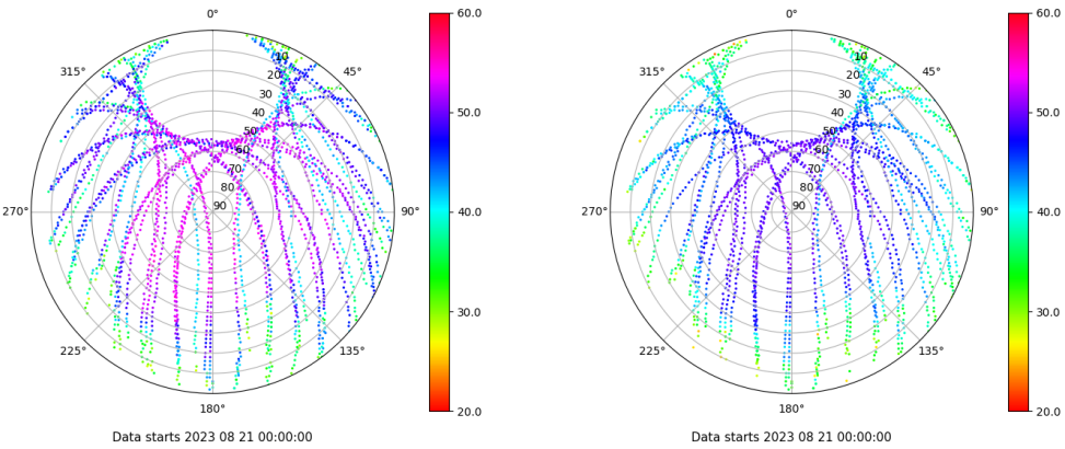
Skyplot for station EIVI. Signal to Noise S1C Data file EIVI00ESP_R_2023233.xtr Skyplot for station EIVI. Signal to Noise S2P Data file EIVI00ESP_R_2023233.xtr
