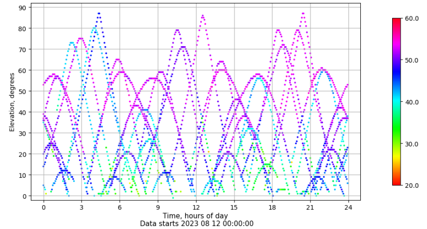
Time-elevation plot for station EIVI. Signal to Noise S1C Data file EIVI00ESP_R_2023224.xtr
