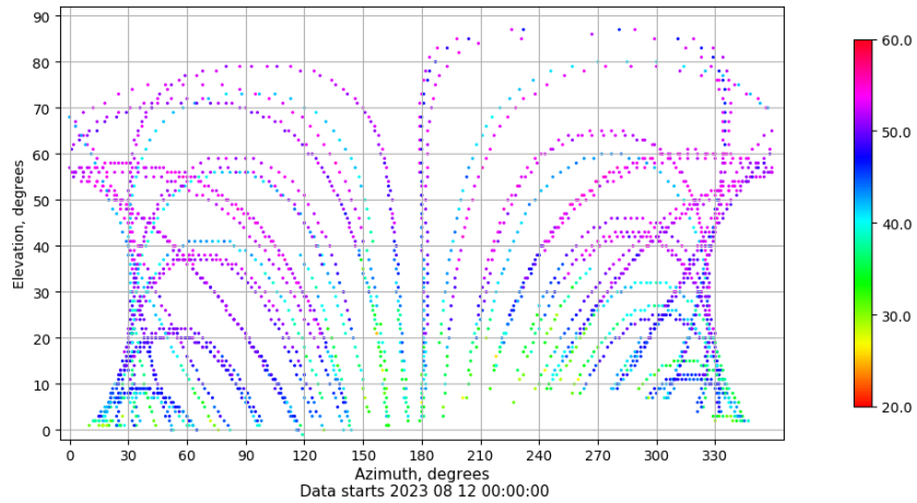
Azimuth-elevation plot for station EIVI. Signal to Noise S1C Data file EIVI00ESP_R_2023224.xtr
