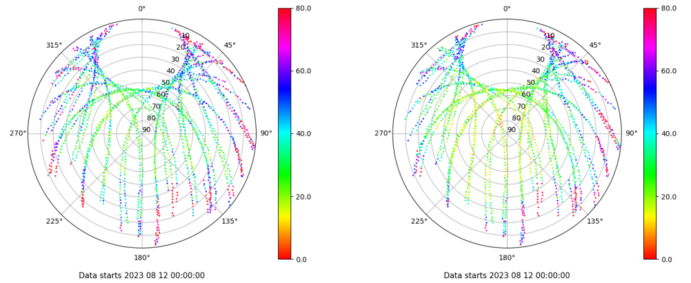
Skyplot for station EIVI. Parameter M1C Data file EIVI00ESP_R_2023224.xtr Skyplot for station EIVI. Parameter M2P Data file EIVI00ESP_R_2023224.xtr
