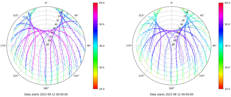
Skyplot for station EIVI. Signal to Noise S1C Data file EIVI00ESP_R_2023224.xtr Skyplot for station EIVI. Signal to Noise S2P Data file EIVI00ESP_R_2023224.xtr
