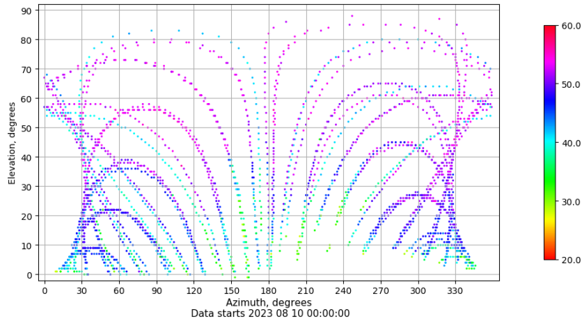
Azimuth-elevation plot for station EIVI. Signal to Noise S1C Data file EIVI00ESP_R_2023222.xtr
