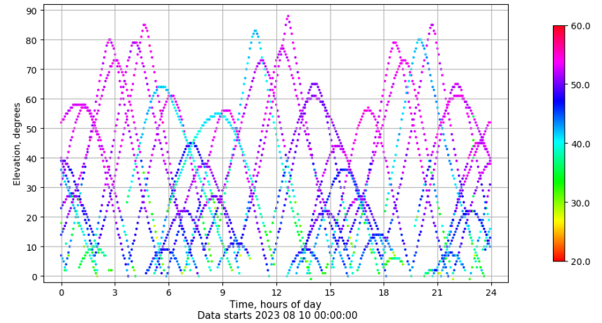
Time-elevation plot for station EIVI. Signal to Noise S1C Data file EIVI00ESP_R_2023222.xtr
