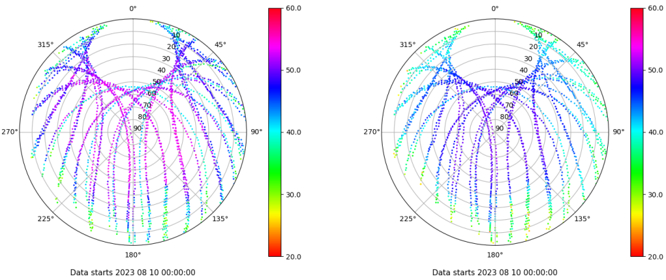
Skyplot for station EIVI. Signal to Noise S1C Data file EIVI00ESP_R_2023222.xtr Skyplot for station EIVI. Signal to Noise S2P Data file EIVI00ESP_R_2023222.xtr
