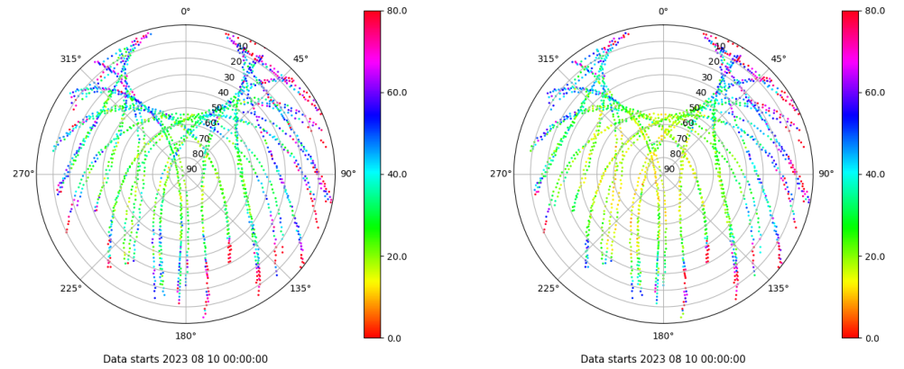
Skyplot for station EIVI. Parameter M1C Data file EIVI00ESP_R_2023222.xtr Skyplot for station EIVI. Parameter M2P Data file EIVI00ESP_R_2023222.xtr
