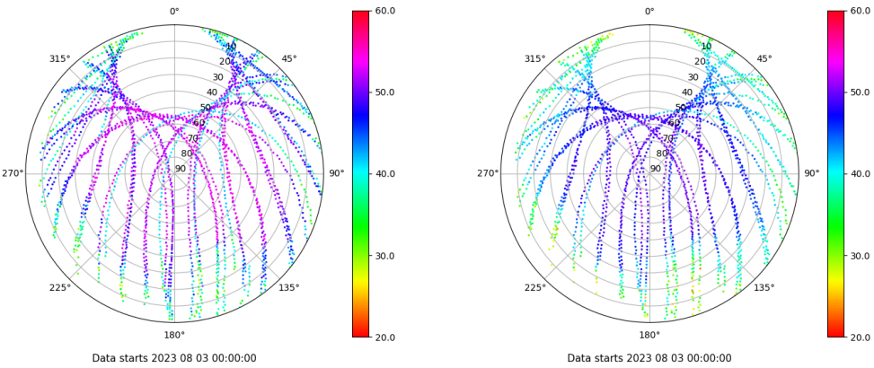
Skyplot for station EIVI. Signal to Noise S1C Data file EIVI00ESP_R_2023215.xtr Skyplot for station EIVI. Signal to Noise S2P Data file EIVI00ESP_R_2023215.xtr
