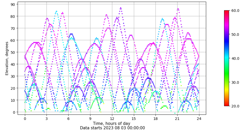
Time-elevation plot for station EIVI. Signal to Noise S1C Data file EIVI00ESP_R_2023215.xtr
