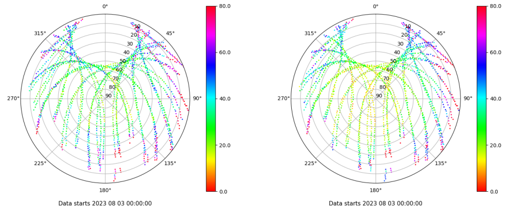
Skyplot for station EIVI. Parameter M1C Data file EIVI00ESP_R_2023215.xtr Skyplot for station EIVI. Parameter M2P Data file EIVI00ESP_R_2023215.xtr
