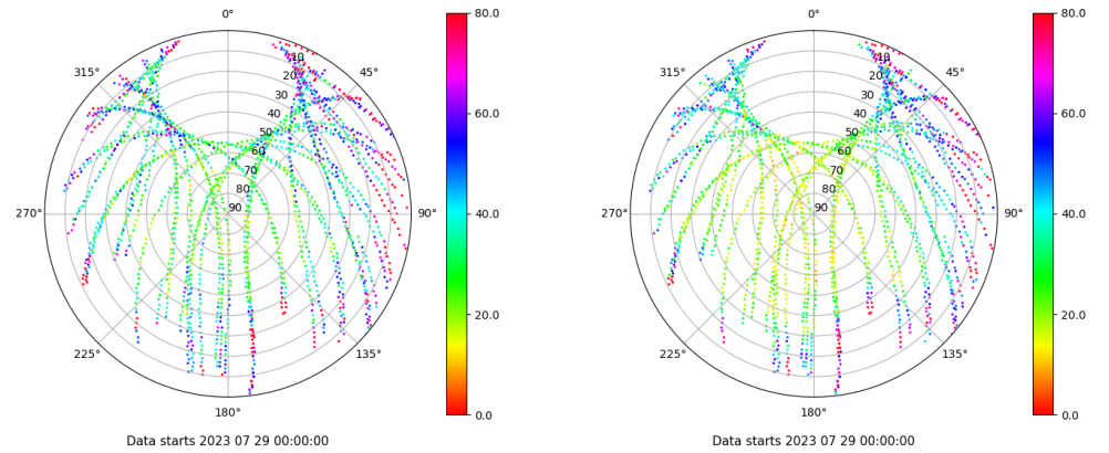
Skyplot for station EIVI. Parameter M1C Data file EIVI00ESP_R_2023210.xtr Skyplot for station EIVI. Parameter M2P Data file EIVI00ESP_R_2023210.xtr
