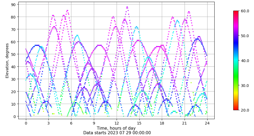
Time-elevation plot for station EIVI. Signal to Noise S1C Data file EIVI00ESP_R_2023210.xtr
