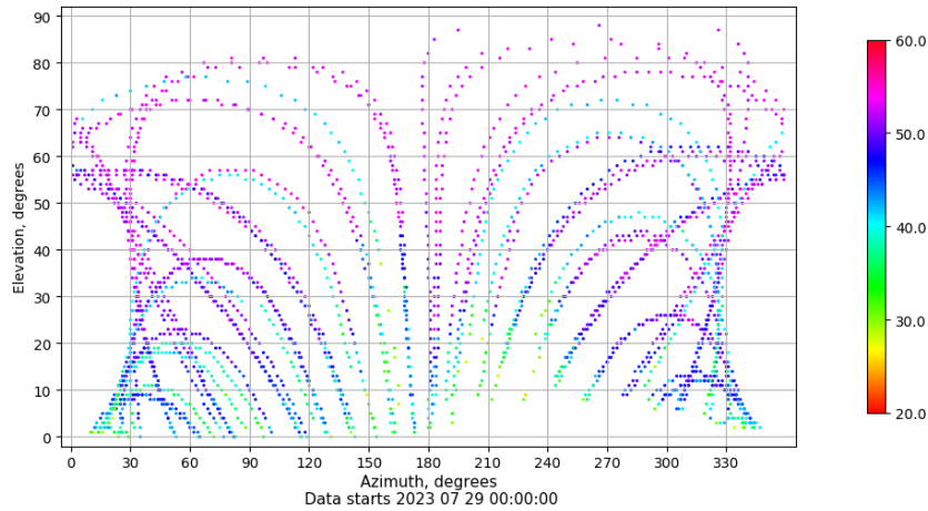
Azimuth-elevation plot for station EIVI. Signal to Noise S1C Data file EIVI00ESP_R_2023210.xtr
