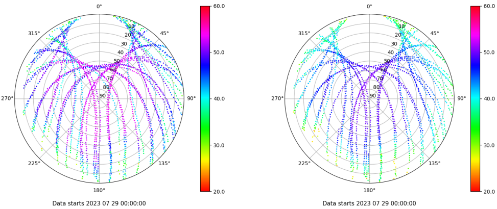
Skyplot for station EIVI. Signal to Noise S1C Data file EIVI00ESP_R_2023210.xtr Skyplot for station EIVI. Signal to Noise S2P Data file EIVI00ESP_R_2023210.xtr
