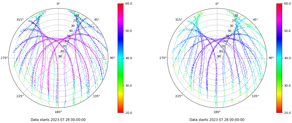
Skyplot for station EIVI. Signal to Noise S1C Data file EIVI00ESP_R_2023209.xtr Skyplot for station EIVI. Signal to Noise S2P Data file EIVI00ESP_R_2023209.xtr
