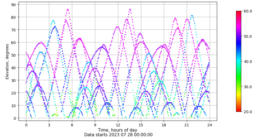
Time-elevation plot for station EIVI. Signal to Noise S1C Data file EIVI00ESP_R_2023209.xtr
