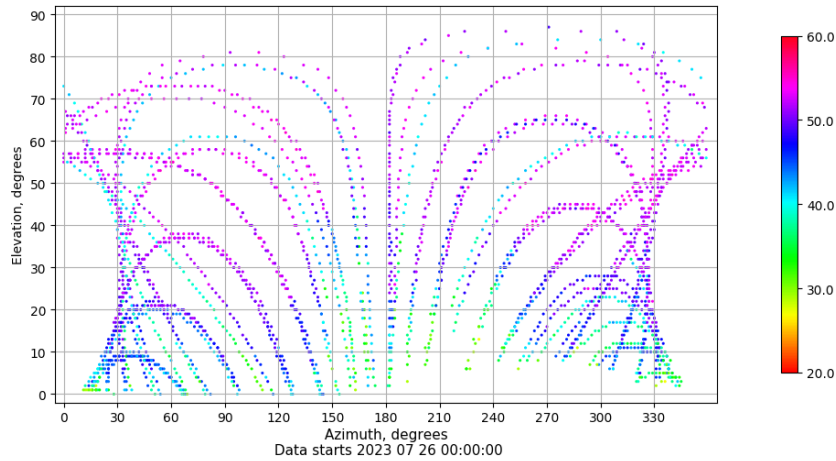
Azimuth-elevation plot for station EIVI. Signal to Noise S1C Data file EIVI00ESP_R_2023207.xtr
