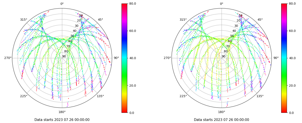
Skyplot for station EIVI. Parameter M1C Data file EIVI00ESP_R_2023207.xtr Skyplot for station EIVI. Parameter M2P Data file EIVI00ESP_R_2023207.xtr
