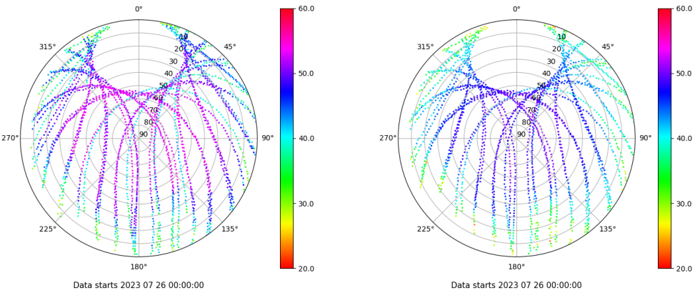
Skyplot for station EIVI. Signal to Noise S1C Data file EIVI00ESP_R_2023207.xtr Skyplot for station EIVI. Signal to Noise S2P Data file EIVI00ESP_R_2023207.xtr
