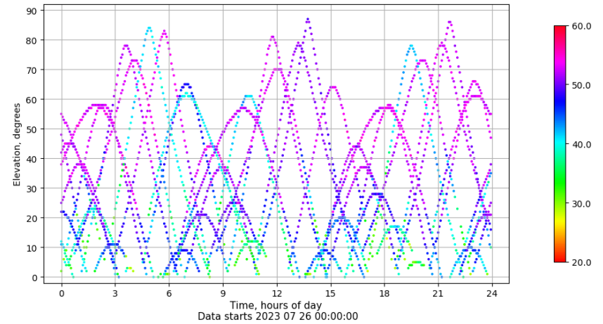
Time-elevation plot for station EIVI. Signal to Noise S1C Data file EIVI00ESP_R_2023207.xtr
