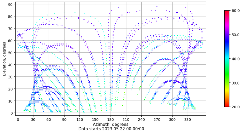
Azimuth-elevation plot for station EIVI. Signal to Noise S1C Data file EIVI00ESP_R_2023142.xtr
