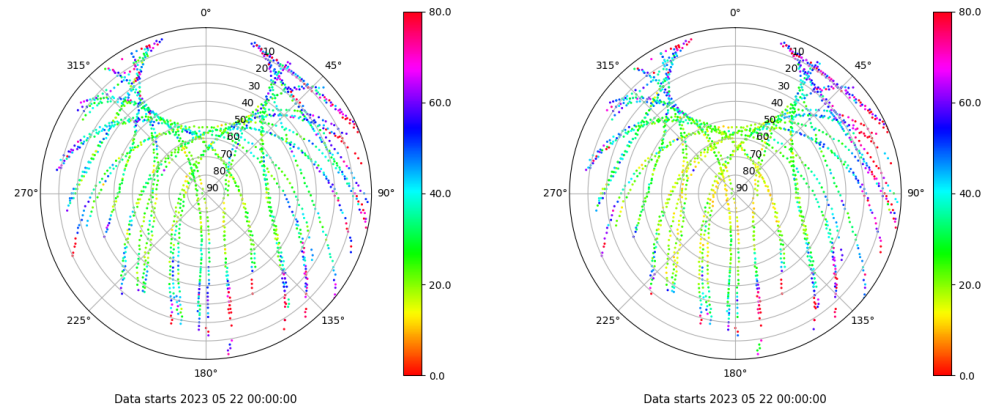
Skyplot for station EIVI. Parameter M1C Data file EIVI00ESP_R_2023142.xtr Skyplot for station EIVI. Parameter M2P Data file EIVI00ESP_R_2023142.xtr
