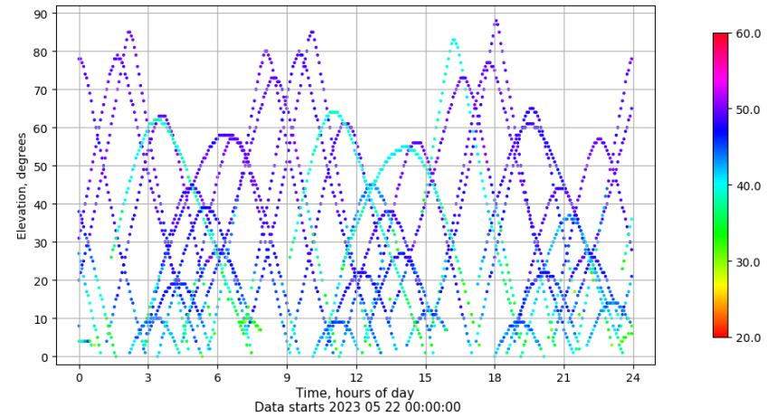
Time-elevation plot for station EIVI. Signal to Noise S1C Data file EIVI00ESP_R_2023142.xtr
