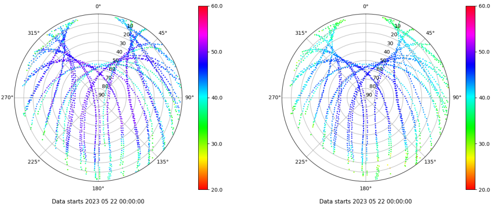
Skyplot for station EIVI. Signal to Noise S1C Data file EIVI00ESP_R_2023142.xtr Skyplot for station EIVI. Signal to Noise S2P Data file EIVI00ESP_R_2023142.xtr
