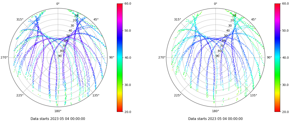
Skyplot for station EIVI. Signal to Noise S1C Data file EIVI00ESP_R_2023124.xtr Skyplot for station EIVI. Signal to Noise S2P Data file EIVI00ESP_R_2023124.xtr
