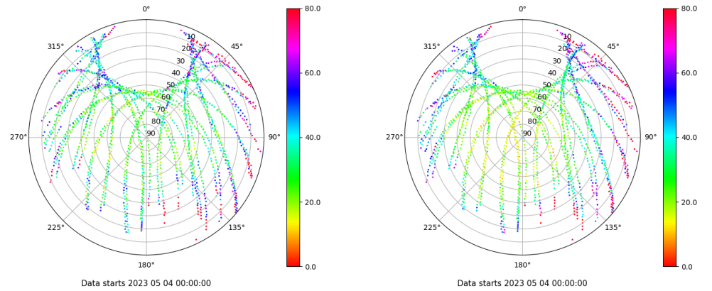
Skyplot for station EIVI. Parameter M1C Data file EIVI00ESP_R_2023124.xtr Skyplot for station EIVI. Parameter M2P Data file EIVI00ESP_R_2023124.xtr
