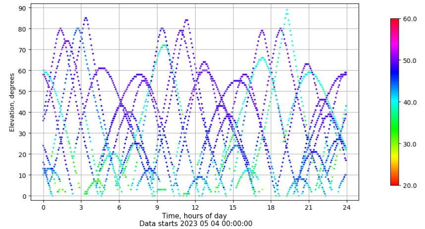
Time-elevation plot for station EIVI. Signal to Noise S1C Data file EIVI00ESP_R_2023124.xtr
