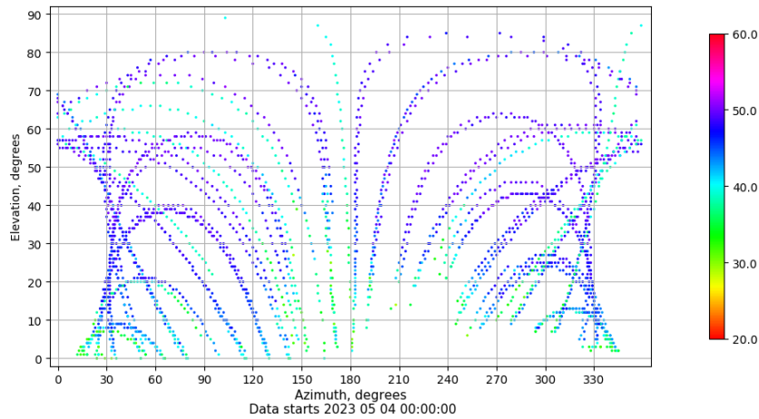
Azimuth-elevation plot for station EIVI. Signal to Noise S1C Data file EIVI00ESP_R_2023124.xtr
