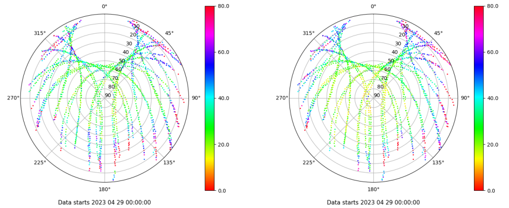
Skyplot for station EIVI. Parameter M1C Data file EIVI00ESP_R_2023119.xtr Skyplot for station EIVI. Parameter M2P Data file EIVI00ESP_R_2023119.xtr
