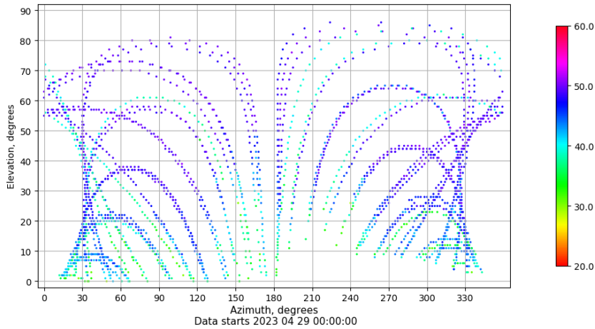
Azimuth-elevation plot for station EIVI. Signal to Noise S1C Data file EIVI00ESP_R_2023119.xtr
