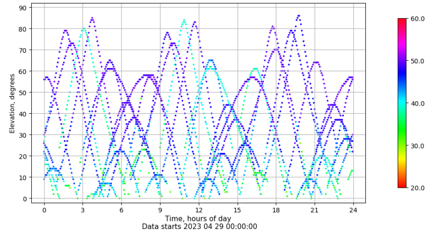
Time-elevation plot for station EIVI. Signal to Noise S1C Data file EIVI00ESP_R_2023119.xtr
