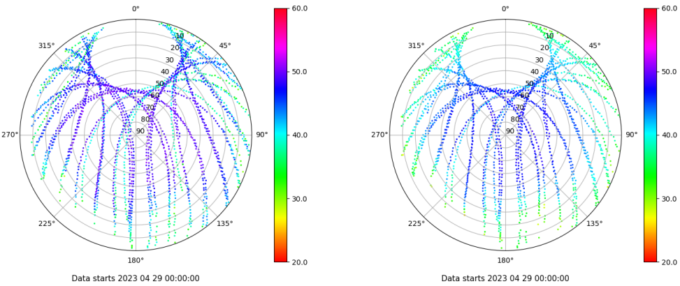
Skyplot for station EIVI. Signal to Noise S1C Data file EIVI00ESP_R_2023119.xtr Skyplot for station EIVI. Signal to Noise S2P Data file EIVI00ESP_R_2023119.xtr
