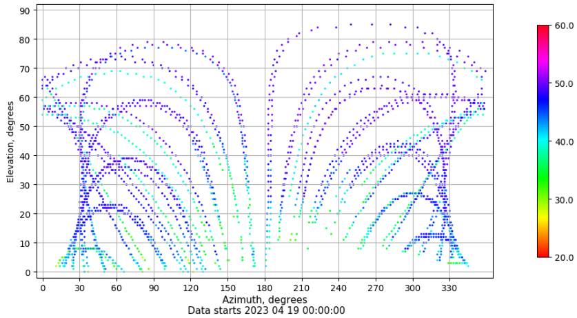
Azimuth-elevation plot for station EIVI. Signal to Noise S1C Data file EIVI00ESP_R_2023109.xtr
