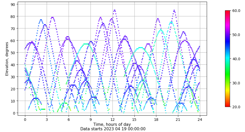
Time-elevation plot for station EIVI. Signal to Noise S1C Data file EIVI00ESP_R_2023109.xtr
