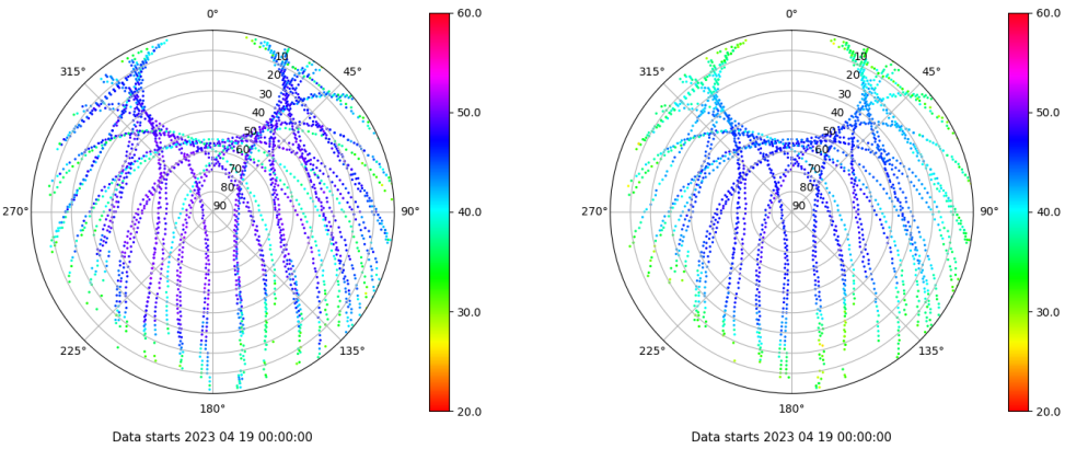
Skyplot for station EIVI. Signal to Noise S1C Data file EIVI00ESP_R_2023109.xtr Skyplot for station EIVI. Signal to Noise S2P Data file EIVI00ESP_R_2023109.xtr
