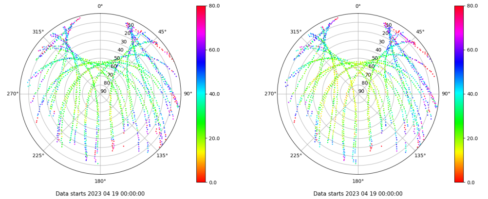
Skyplot for station EIVI. Parameter M1C Data file EIVI00ESP_R_2023109.xtr Skyplot for station EIVI. Parameter M2P Data file EIVI00ESP_R_2023109.xtr
