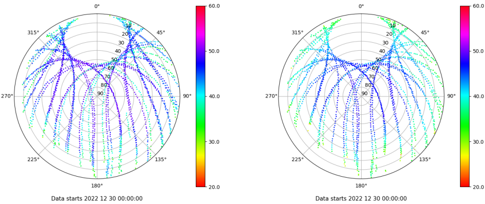
Skyplot for station EIVI. Signal to Noise S1C Data file EIVI00ESP_R_2022364.xtr Skyplot for station EIVI. Signal to Noise S2P Data file EIVI00ESP_R_2022364.xtr
