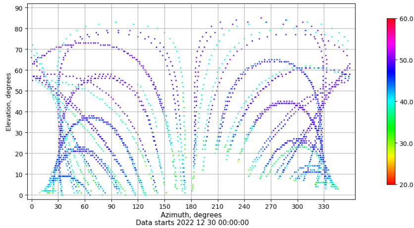
Azimuth-elevation plot for station EIVI. Signal to Noise S1C Data file EIVI00ESP_R_2022364.xtr
