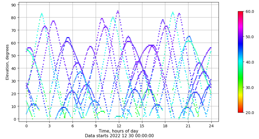
Time-elevation plot for station EIVI. Signal to Noise S1C Data file EIVI00ESP_R_2022364.xtr
