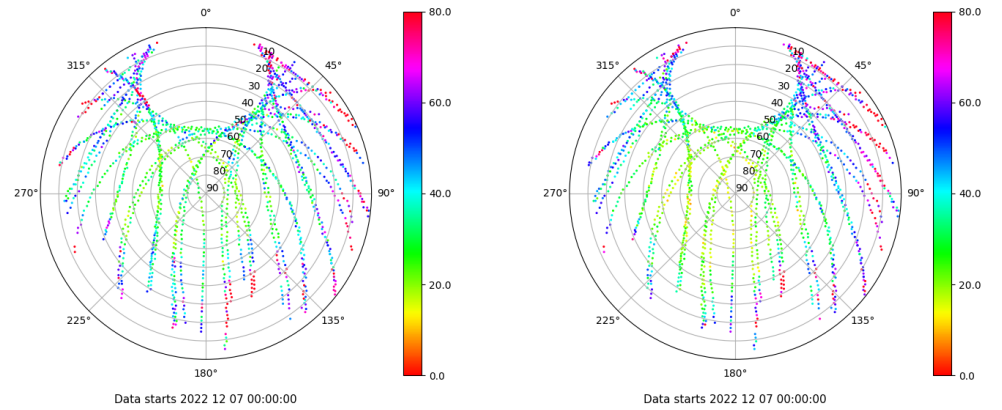
Skyplot for station EIVI. Parameter M1C Data file EIVI00ESP_R_2022341.xtr Skyplot for station EIVI. Parameter M2P Data file EIVI00ESP_R_2022341.xtr
