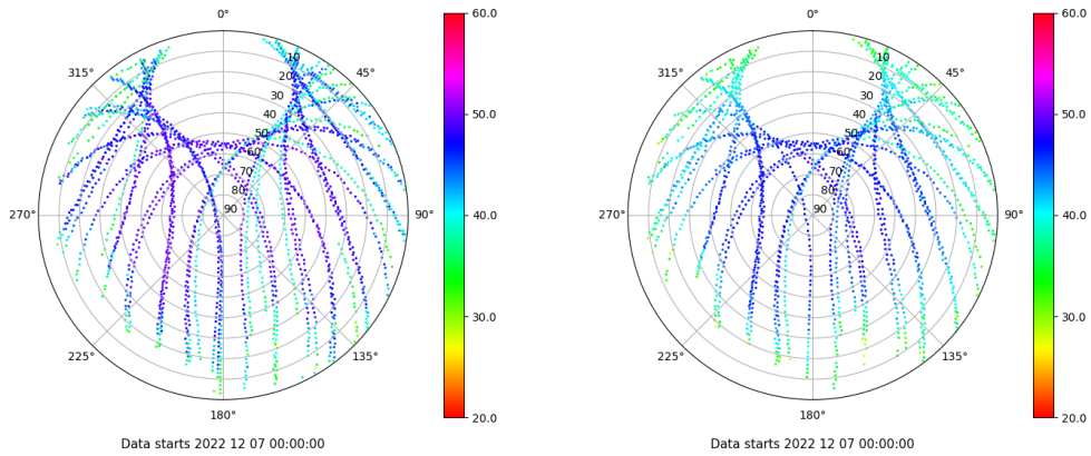
Skyplot for station EIVI. Signal to Noise S1C Data file EIVI00ESP_R_2022341.xtr Skyplot for station EIVI. Signal to Noise S2P Data file EIVI00ESP_R_2022341.xtr
