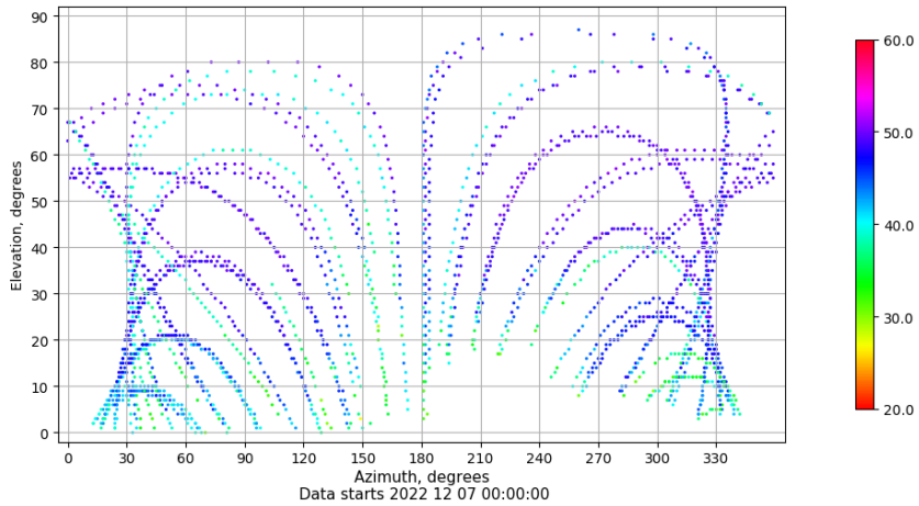
Azimuth-elevation plot for station EIVI. Signal to Noise S1C Data file EIVI00ESP_R_2022341.xtr
