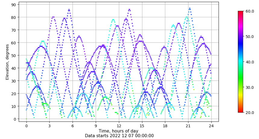
Time-elevation plot for station EIVI. Signal to Noise S1C Data file EIVI00ESP_R_2022341.xtr
