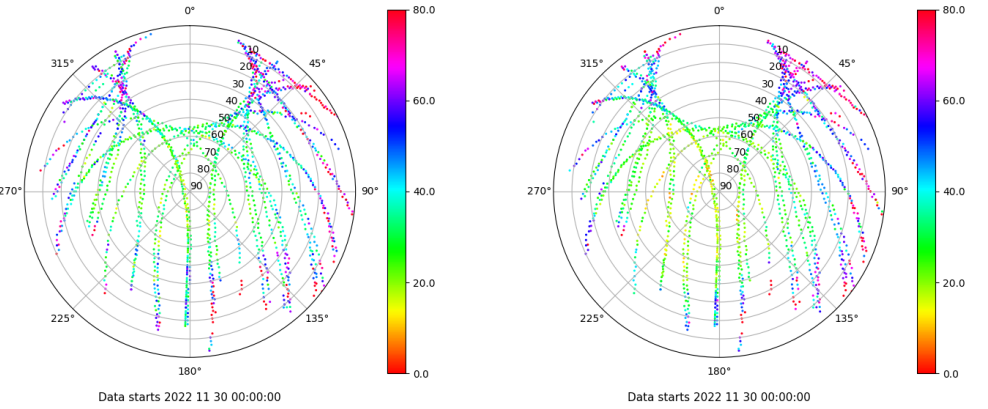
Skyplot for station EIVI. Parameter M1C Data file EIVI00ESP_R_2022334.xtr Skyplot for station EIVI. Parameter M2P Data file EIVI00ESP_R_2022334.xtr
