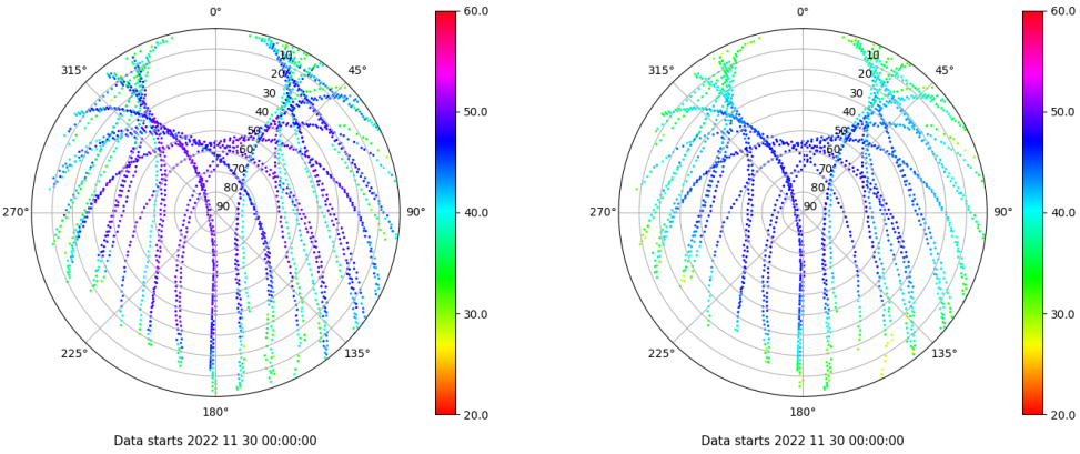
Skyplot for station EIVI. Signal to Noise S1C Data file EIVI00ESP_R_2022334.xtr Skyplot for station EIVI. Signal to Noise S2P Data file EIVI00ESP_R_2022334.xtr
