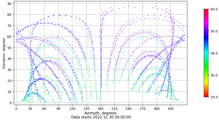
Azimuth-elevation plot for station EIVI. Signal to Noise S1C Data file EIVI00ESP_R_2022334.xtr
