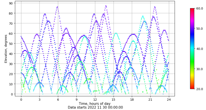
Time-elevation plot for station EIVI. Signal to Noise S1C Data file EIVI00ESP_R_2022334.xtr
