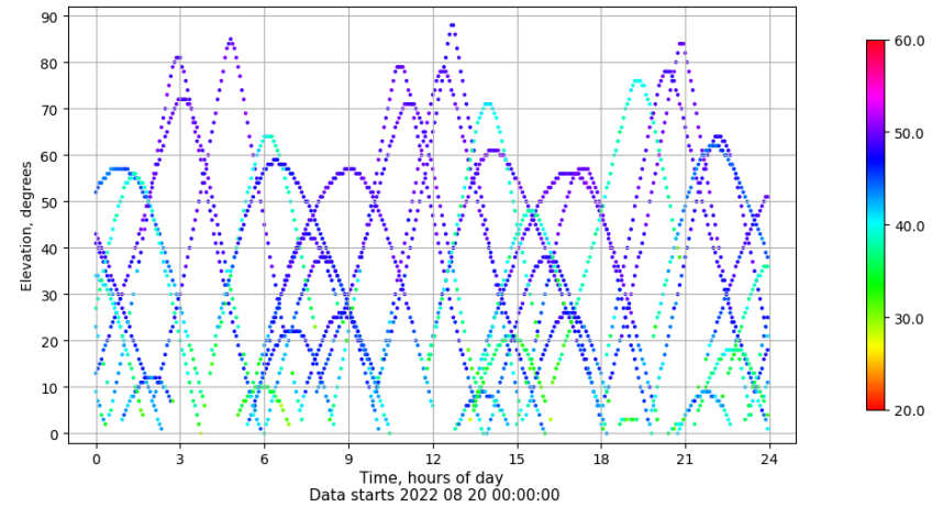
Time-elevation plot for station EIVI. Signal to Noise S1C Data file EIVI00ESP_R_2022232.xtr
