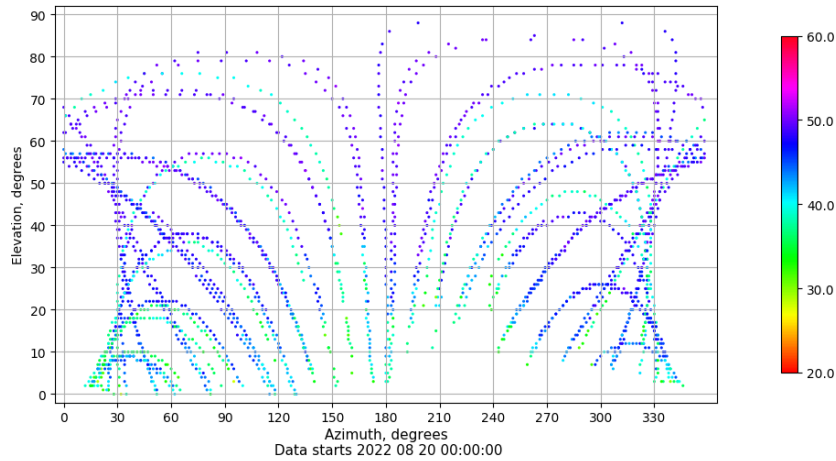
Azimuth-elevation plot for station EIVI. Signal to Noise S1C Data file EIVI00ESP_R_2022232.xtr
