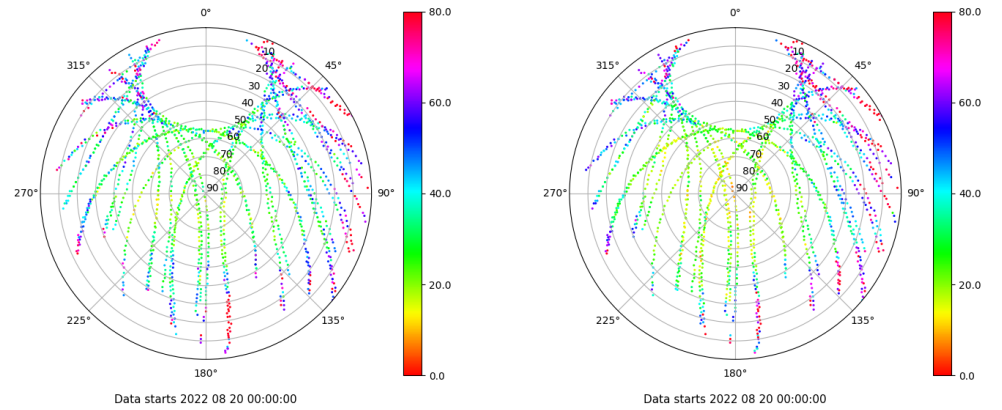
Skyplot for station EIVI. Parameter M1C Data file EIVI00ESP_R_2022232.xtr Skyplot for station EIVI. Parameter M2P Data file EIVI00ESP_R_2022232.xtr
