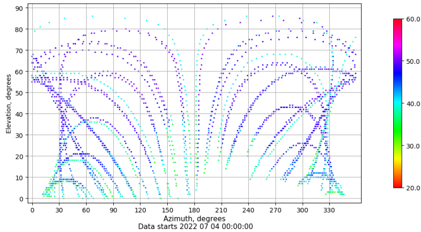
Azimuth-elevation plot for station EIVI. Signal to Noise S1C Data file EIVI00ESP_R_2022185.xtr
