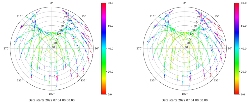
Skyplot for station EIVI. Parameter M1C Data file EIVI00ESP_R_2022185.xtr Skyplot for station EIVI. Parameter M2P Data file EIVI00ESP_R_2022185.xtr
