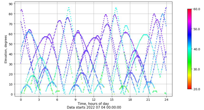
Time-elevation plot for station EIVI. Signal to Noise S1C Data file EIVI00ESP_R_2022185.xtr
