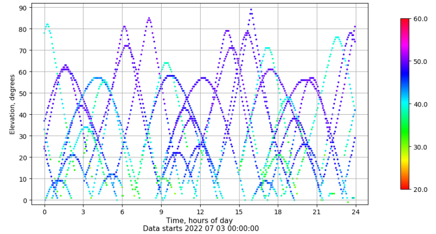
Time-elevation plot for station EIVI. Signal to Noise S1C Data file EIVI00ESP_R_2022184.xtr
