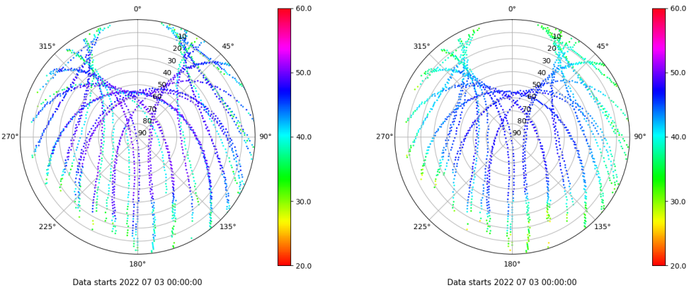
Skyplot for station EIVI. Signal to Noise S1C Data file EIVI00ESP_R_2022184.xtr Skyplot for station EIVI. Signal to Noise S2P Data file EIVI00ESP_R_2022184.xtr
