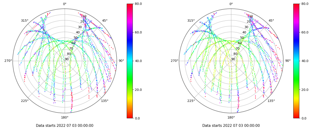
Skyplot for station EIVI. Parameter M1C Data file EIVI00ESP_R_2022184.xtr Skyplot for station EIVI. Parameter M2P Data file EIVI00ESP_R_2022184.xtr
