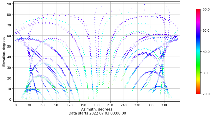
Azimuth-elevation plot for station EIVI. Signal to Noise S1C Data file EIVI00ESP_R_2022184.xtr
