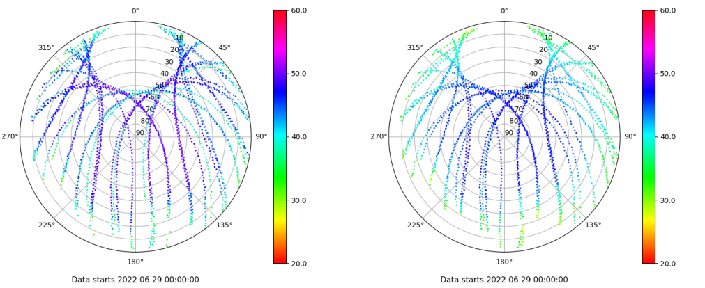
Skyplot for station EIVI. Signal to Noise S1C Data file EIVI00ESP_R_2022180.xtr Skyplot for station EIVI. Signal to Noise S2P Data file EIVI00ESP_R_2022180.xtr
