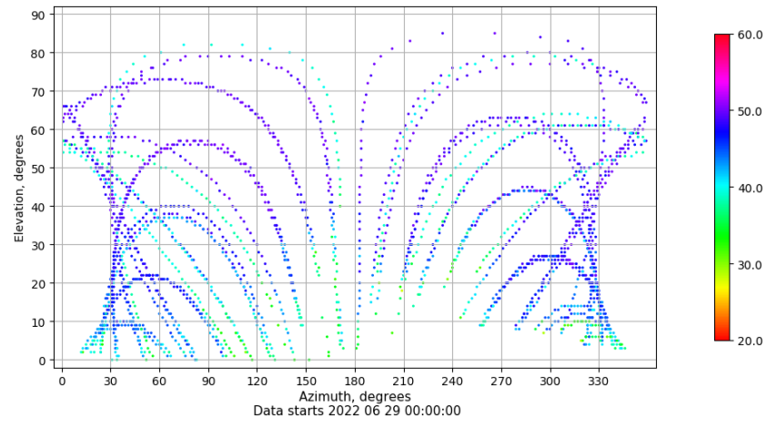
Azimuth-elevation plot for station EIVI. Signal to Noise S1C Data file EIVI00ESP_R_2022180.xtr
