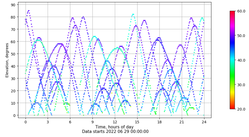
Time-elevation plot for station EIVI. Signal to Noise S1C Data file EIVI00ESP_R_2022180.xtr
