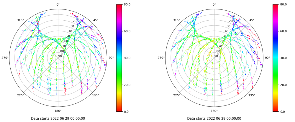
Skyplot for station EIVI. Parameter M1C Data file EIVI00ESP_R_2022180.xtr Skyplot for station EIVI. Parameter M2P Data file EIVI00ESP_R_2022180.xtr
