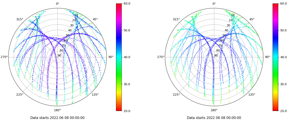
Skyplot for station EIVI. Signal to Noise S1C Data file EIVI00ESP_R_2022159.xtr Skyplot for station EIVI. Signal to Noise S2P Data file EIVI00ESP_R_2022159.xtr
