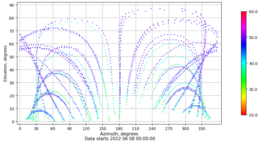
Azimuth-elevation plot for station EIVI. Signal to Noise S1C Data file EIVI00ESP_R_2022159.xtr
