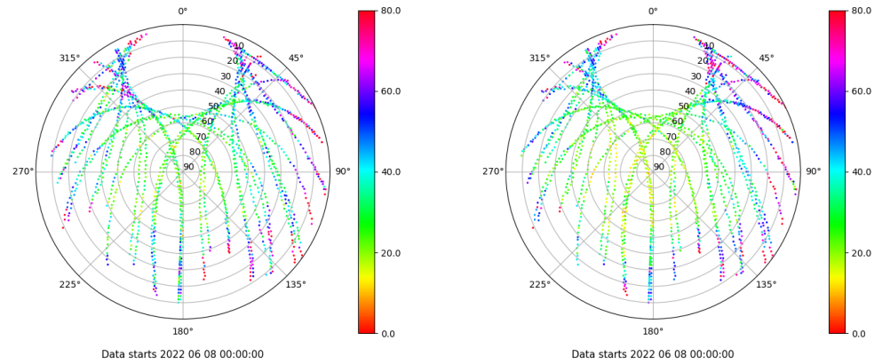
Skyplot for station EIVI. Parameter M1C Data file EIVI00ESP_R_2022159.xtr Skyplot for station EIVI. Parameter M2P Data file EIVI00ESP_R_2022159.xtr
