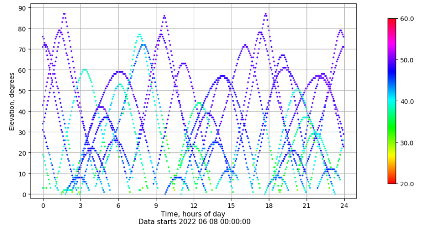
Time-elevation plot for station EIVI. Signal to Noise S1C Data file EIVI00ESP_R_2022159.xtr
