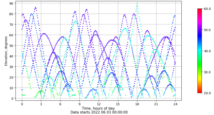
Time-elevation plot for station EIVI. Signal to Noise S1C Data file EIVI00ESP_R_2022154.xtr
