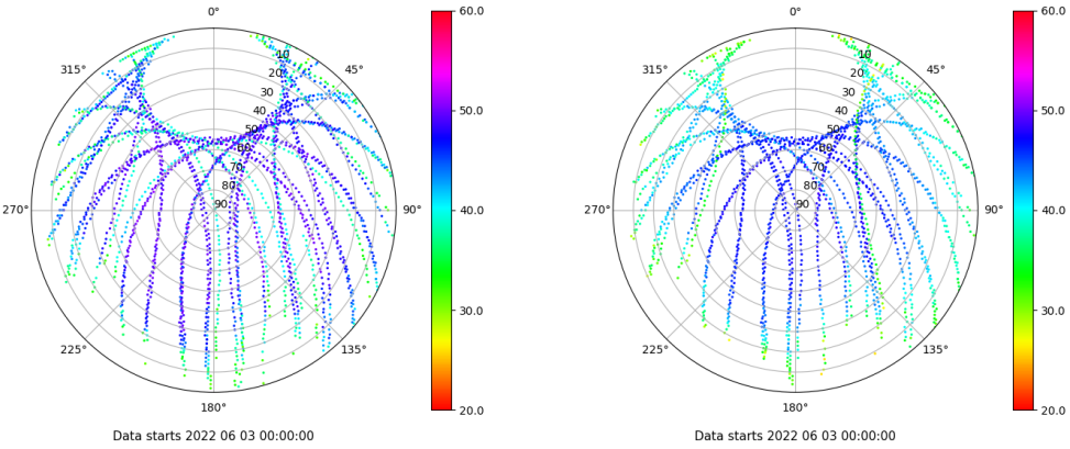
Skyplot for station EIVI. Signal to Noise S1C Data file EIVI00ESP_R_2022154.xtr Skyplot for station EIVI. Signal to Noise S2P Data file EIVI00ESP_R_2022154.xtr
