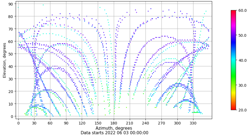
Azimuth-elevation plot for station EIVI. Signal to Noise S1C Data file EIVI00ESP_R_2022154.xtr
