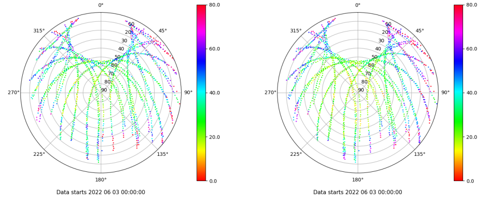
Skyplot for station EIVI. Parameter M1C Data file EIVI00ESP_R_2022154.xtr Skyplot for station EIVI. Parameter M2P Data file EIVI00ESP_R_2022154.xtr
