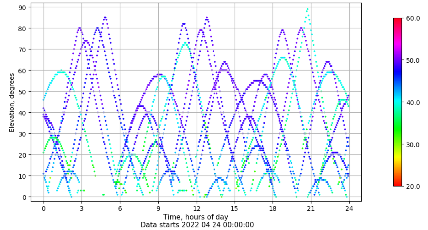
Time-elevation plot for station EIVI. Signal to Noise S1C Data file EIVI00ESP_R_2022114.xtr
