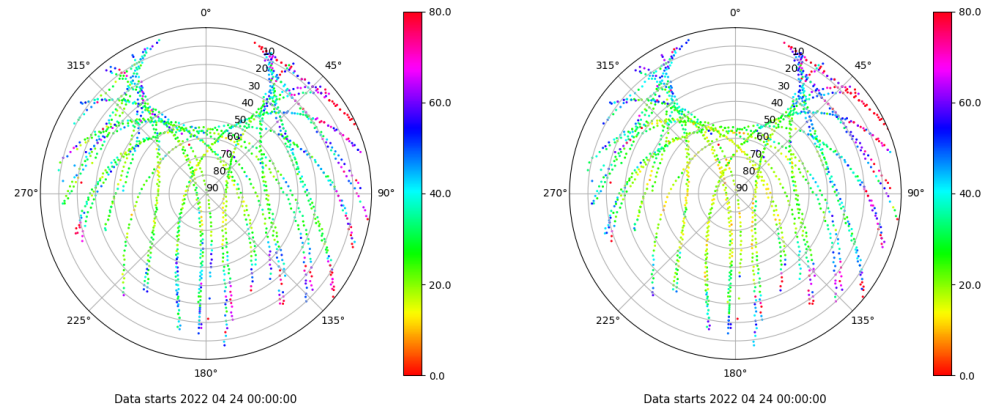
Skyplot for station EIVI. Parameter M1C Data file EIVI00ESP_R_2022114.xtr Skyplot for station EIVI. Parameter M2P Data file EIVI00ESP_R_2022114.xtr
