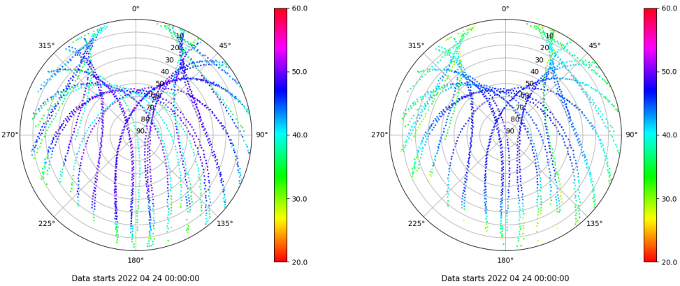
Skyplot for station EIVI. Signal to Noise S1C Data file EIVI00ESP_R_2022114.xtr Skyplot for station EIVI. Signal to Noise S2P Data file EIVI00ESP_R_2022114.xtr
