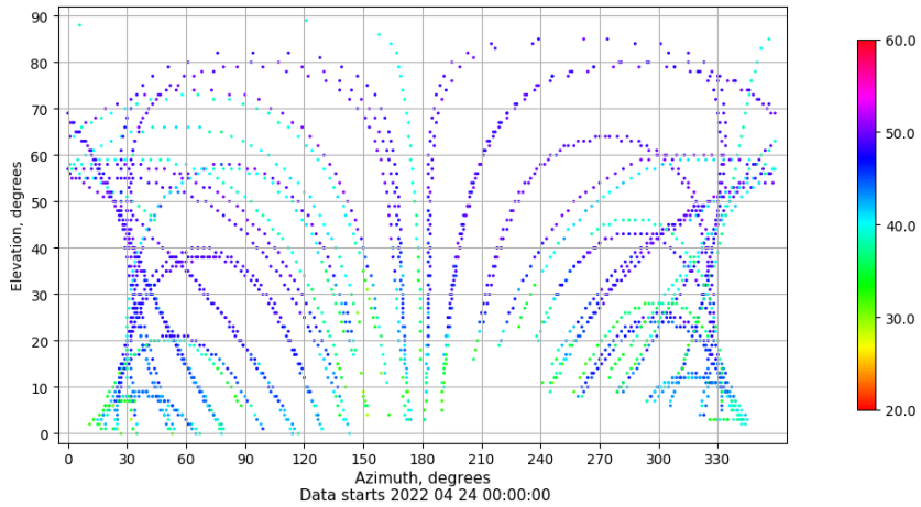
Azimuth-elevation plot for station EIVI. Signal to Noise S1C Data file EIVI00ESP_R_2022114.xtr
