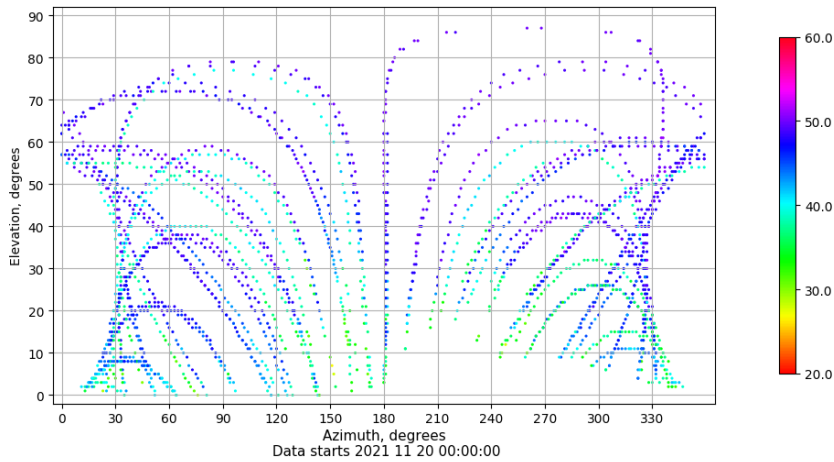
Azimuth-elevation plot for station EIVI. Signal to Noise S1C Data file EIVI00ESP_R_2021324.xtr
