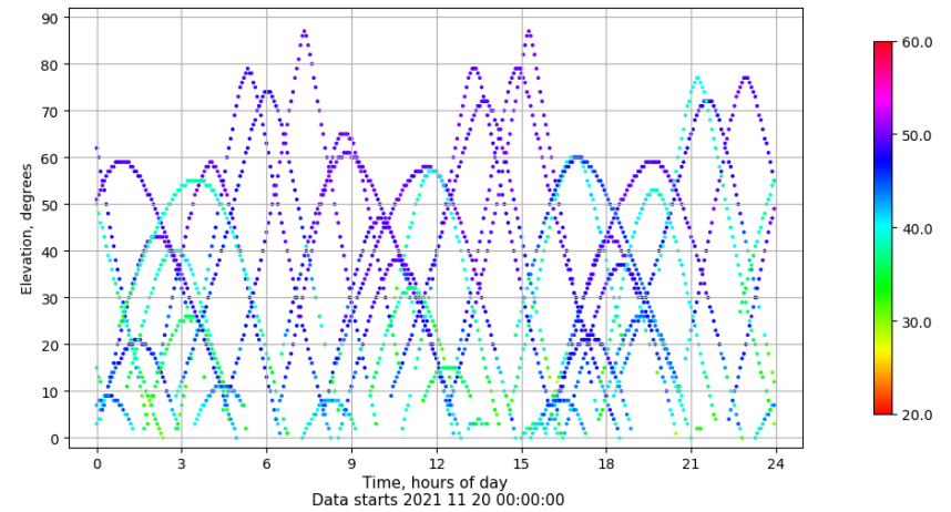
Time-elevation plot for station EIVI. Signal to Noise S1C Data file EIVI00ESP_R_2021324.xtr
