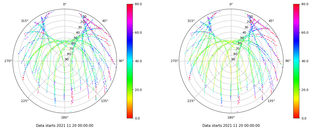
Skyplot for station EIVI. Parameter M1C Data file EIVI00ESP_R_2021324.xtr Skyplot for station EIVI. Parameter M2P Data file EIVI00ESP_R_2021324.xtr
