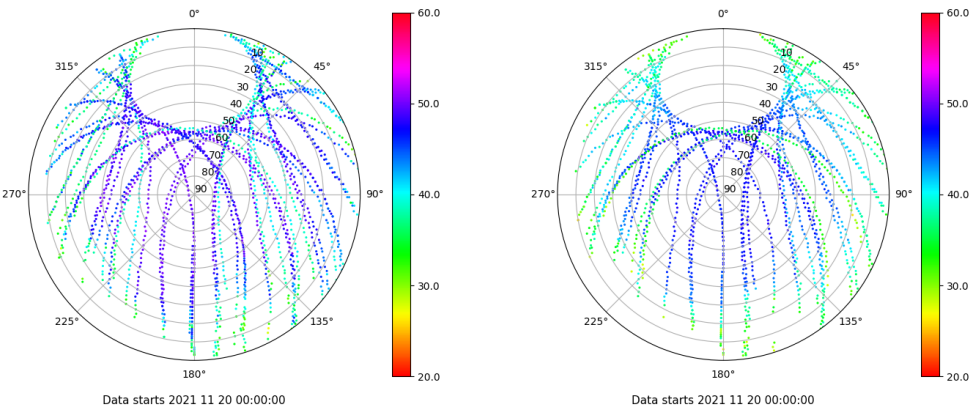
Skyplot for station EIVI. Signal to Noise S1C Data file EIVI00ESP_R_2021324.xtr Skyplot for station EIVI. Signal to Noise S2P Data file EIVI00ESP_R_2021324.xtr
