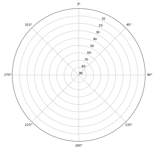
Skyplot for station EIVI. Parameter M5Q Data file EIVI00ESP_R_2021316.xtr
