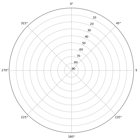
Skyplot for station EIVI. Parameter M1C Data file EIVI00ESP_R_2021316.xtr
