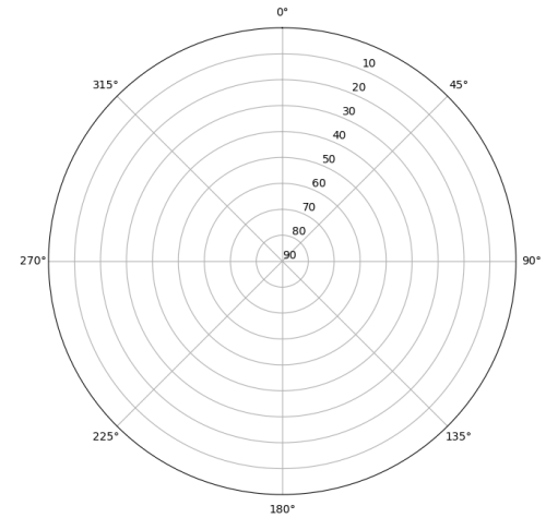
Skyplot for station EIVI. Parameter M2P Data file EIVI00ESP_R_2021316.xtr
