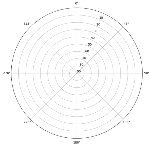
Skyplot for station EIVI. Signal to Noise S2P Data file EIVI00ESP_R_2021316.xtr
