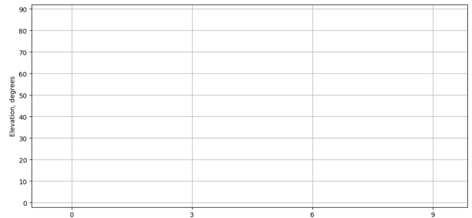
Time-elevation plot for station EIVI. Signal to Noise S1C Data file EIVI00ESP_R_2021316.xtr
