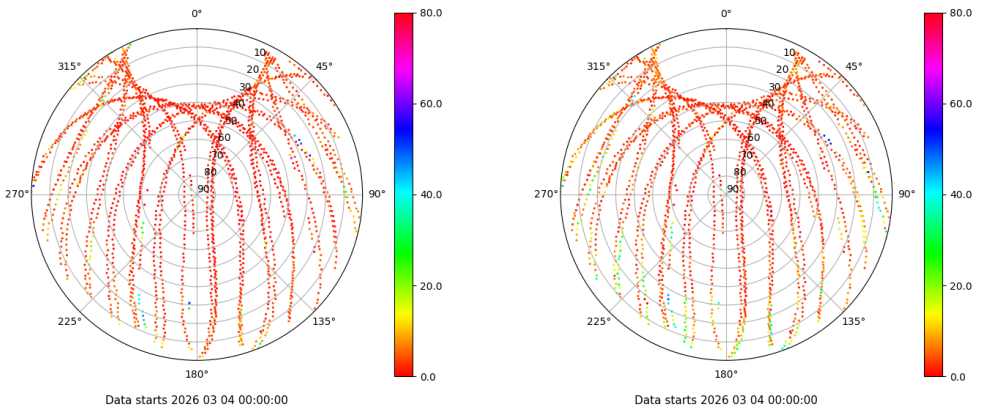
Skyplot for station EH01. Parameter M1C Data file EH0100ESP_R_2026063.xtr Skyplot for station EH01. Parameter M2P Data file EH0100ESP_R_2026063.xtr
