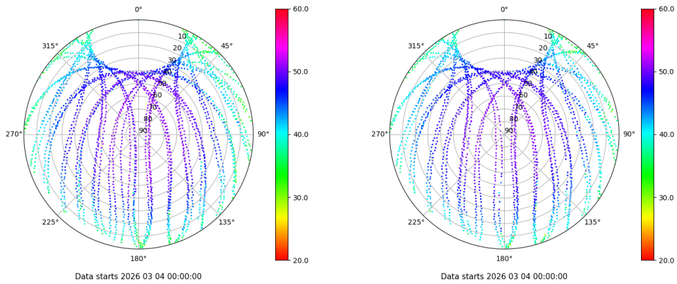
Skyplot for station EH01. Signal to Noise S1C Data file EH0100ESP_R_2026063.xtr Skyplot for station EH01. Signal to Noise S2P Data file EH0100ESP_R_2026063.xtr
