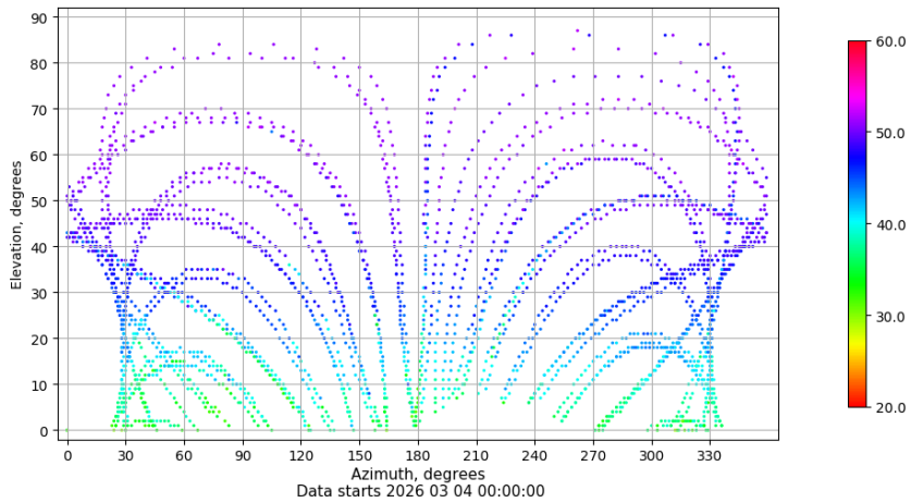
Azimuth-elevation plot for station EH01. Signal to Noise S1C Data file EH0100ESP_R_2026063.xtr
