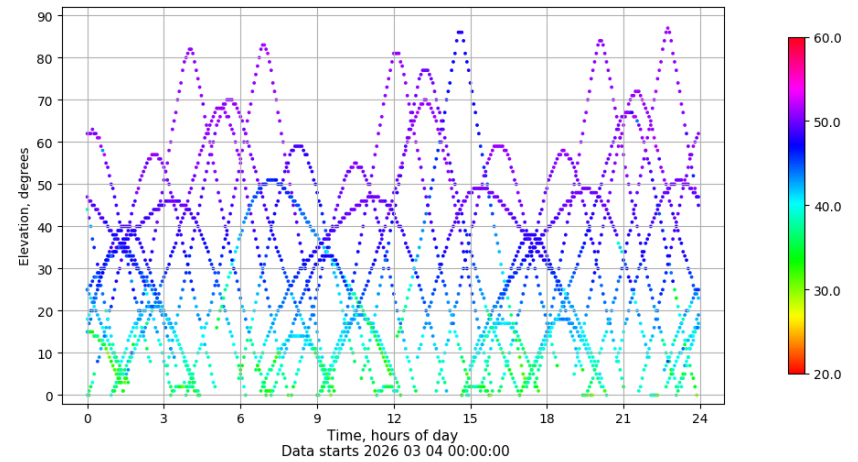
Time-elevation plot for station EH01. Signal to Noise S1C Data file EH0100ESP_R_2026063.xtr
