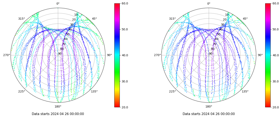
Skyplot for station EH01. Signal to Noise S1C Data file EH0100ESP_R_2024117.xtr Skyplot for station EH01. Signal to Noise S2P Data file EH0100ESP_R_2024117.xtr
