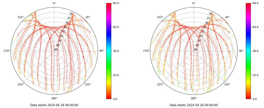
Skyplot for station EH01. Parameter M1C Data file EH0100ESP_R_2024117.xtr Skyplot for station EH01. Parameter M2P Data file EH0100ESP_R_2024117.xtr
