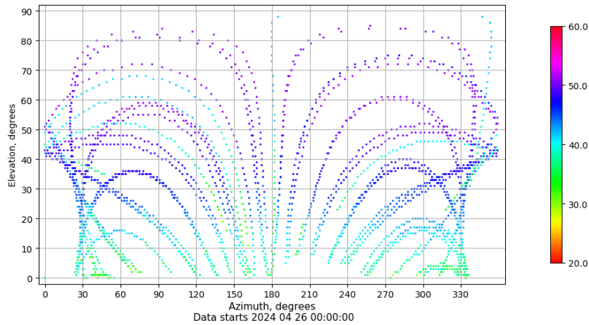
Azimuth-elevation plot for station EH01. Signal to Noise S1C Data file EH0100ESP_R_2024117.xtr
