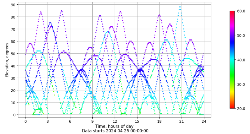
Time-elevation plot for station EH01. Signal to Noise S1C Data file EH0100ESP_R_2024117.xtr
