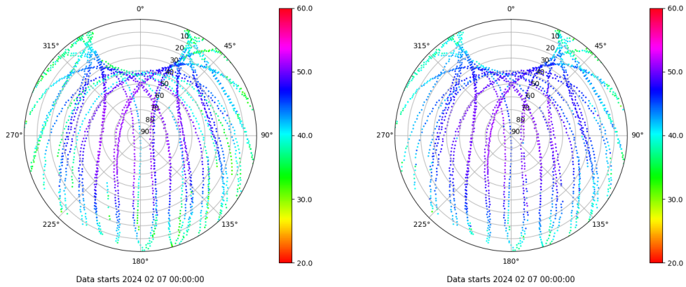
Skyplot for station EH01. Signal to Noise S1C Data file EH0100ESP_R_2024038.xtr Skyplot for station EH01. Signal to Noise S2P Data file EH0100ESP_R_2024038.xtr
