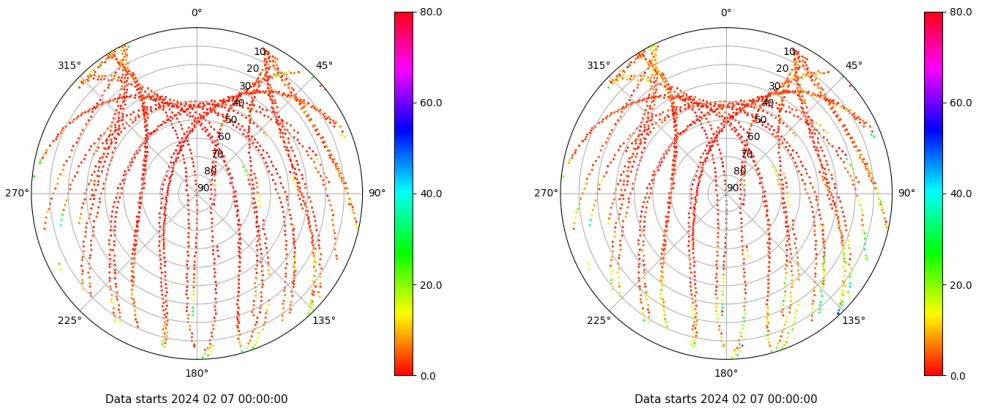
Skyplot for station EH01. Parameter M1C Data file EH0100ESP_R_2024038.xtr Skyplot for station EH01. Parameter M2P Data file EH0100ESP_R_2024038.xtr
