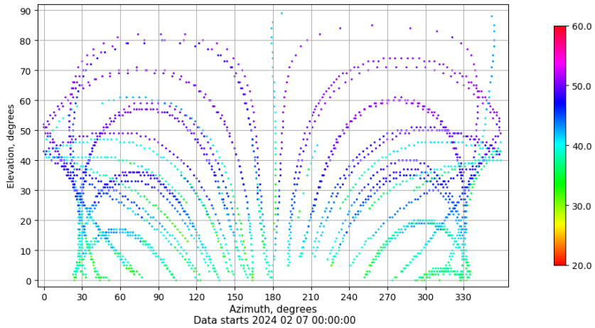
Azimuth-elevation plot for station EH01. Signal to Noise S1C Data file EH0100ESP_R_2024038.xtr
