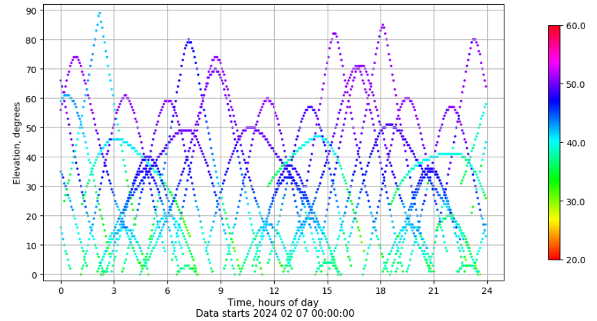
Time-elevation plot for station EH01. Signal to Noise S1C Data file EH0100ESP_R_2024038.xtr
