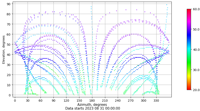
Azimuth-elevation plot for station EH01. Signal to Noise S1C Data file EH0100ESP_R_2023243.xtr
