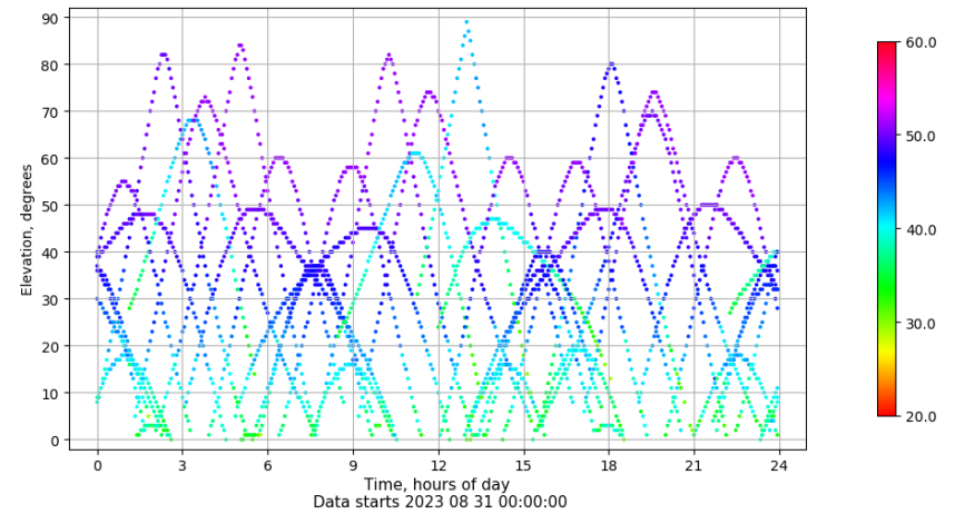
Time-elevation plot for station EH01. Signal to Noise S1C Data file EH0100ESP_R_2023243.xtr
