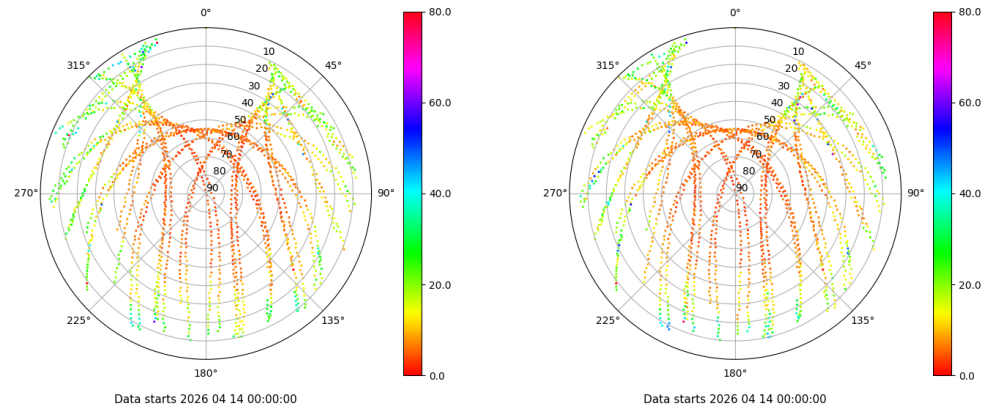
Skyplot for station CLTR. Parameter M1C Data file CLTR00ESP_R_2026104.xtr Skyplot for station CLTR. Parameter M2P Data file CLTR00ESP_R_2026104.xtr
