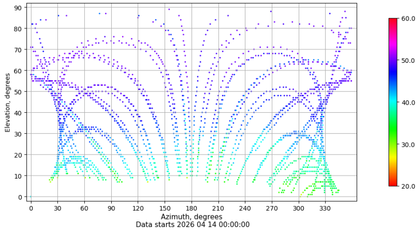
Azimuth-elevation plot for station CLTR. Signal to Noise S1C Data file CLTR00ESP_R_2026104.xtr
