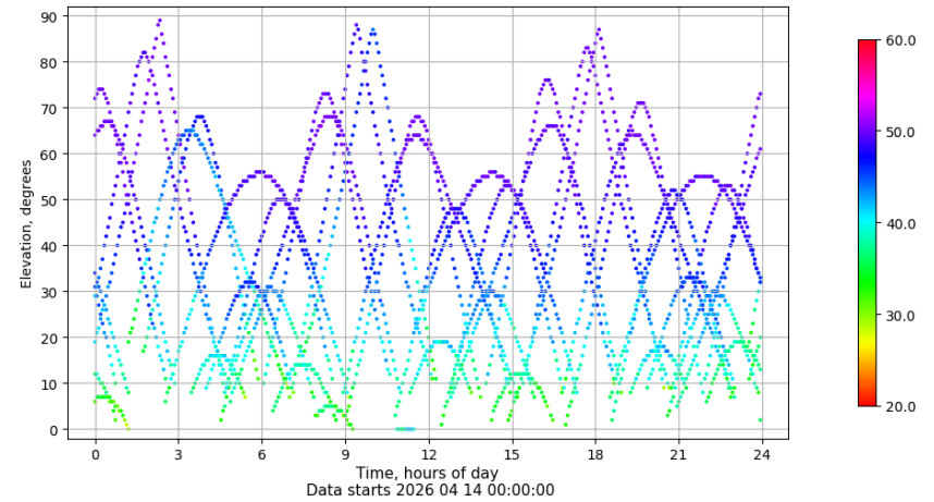
Time-elevation plot for station CLTR. Signal to Noise S1C Data file CLTR00ESP_R_2026104.xtr
