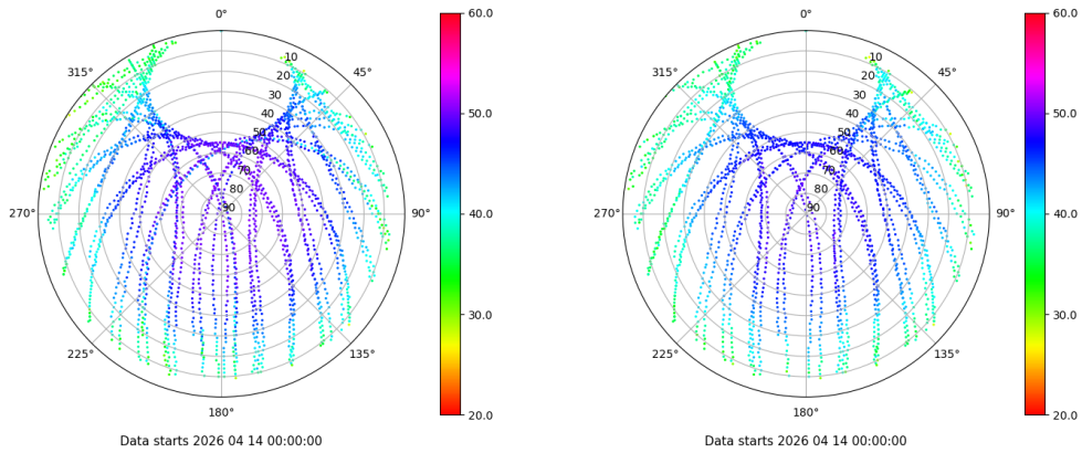
Skyplot for station CLTR. Signal to Noise S1C Data file CLTR00ESP_R_2026104.xtr Skyplot for station CLTR. Signal to Noise S2P Data file CLTR00ESP_R_2026104.xtr
