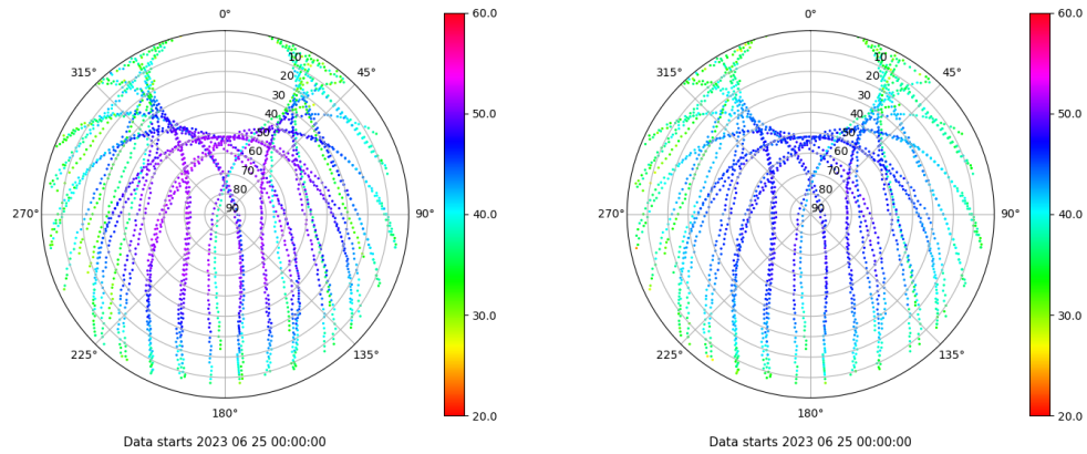
Skyplot for station CEU1. Signal to Noise S1C Data file CEU100ESP_R_2023176.xtr Skyplot for station CEU1. Signal to Noise S2C Data file CEU100ESP_R_2023176.xtr
