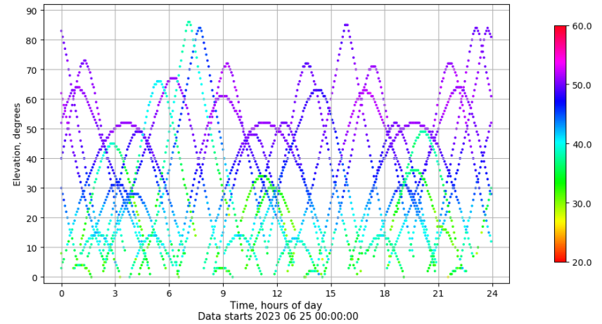
Time-elevation plot for station CEU1. Signal to Noise S1C Data file CEU100ESP_R_2023176.xtr
