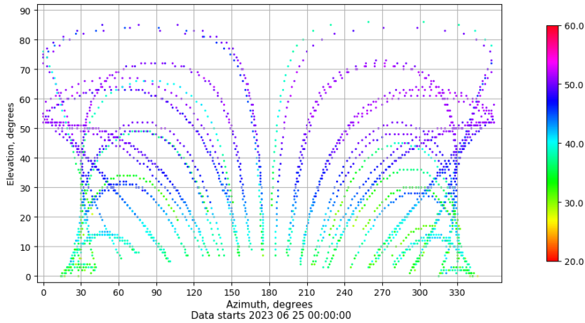
Azimuth-elevation plot for station CEU1. Signal to Noise S1C Data file CEU100ESP_R_2023176.xtr
