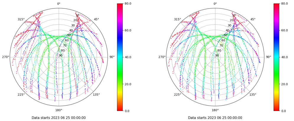
Skyplot for station CEU1. Parameter M1C Data file CEU100ESP_R_2023176.xtr Skyplot for station CEU1. Parameter M2C Data file CEU100ESP_R_2023176.xtr
