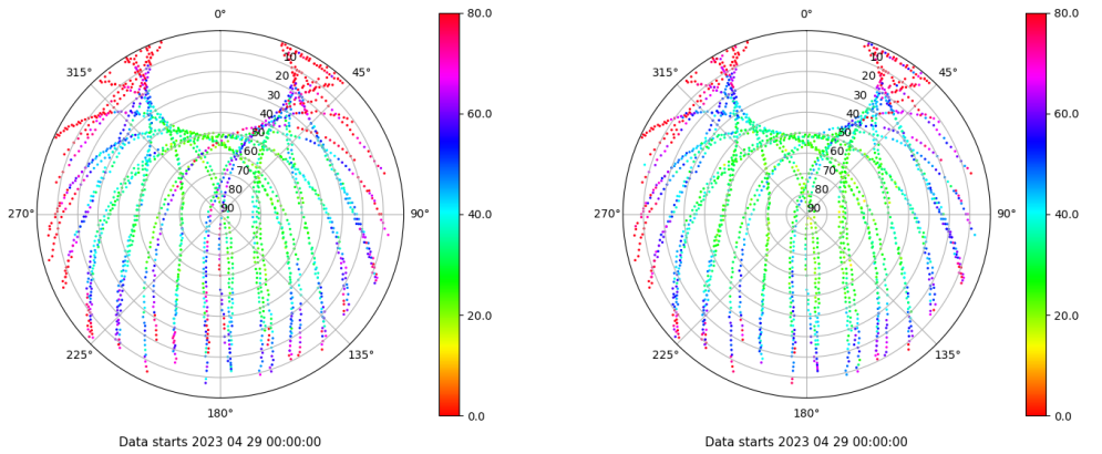
Skyplot for station CEU1. Parameter M1C Data file CEU100ESP_R_2023119.xtr Skyplot for station CEU1. Parameter M2C Data file CEU100ESP_R_2023119.xtr
