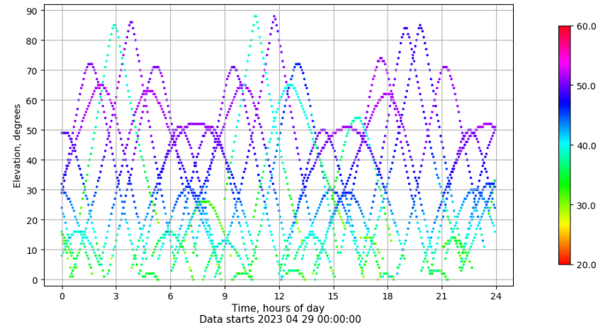
Time-elevation plot for station CEU1. Signal to Noise S1C Data file CEU100ESP_R_2023119.xtr
