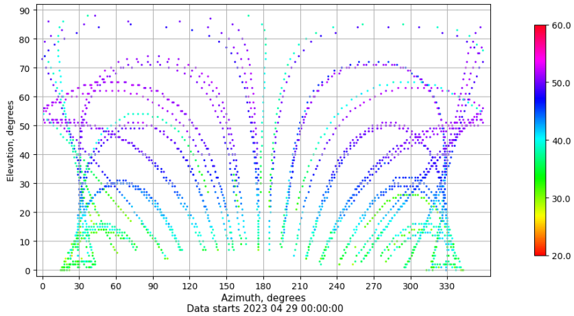
Azimuth-elevation plot for station CEU1. Signal to Noise S1C Data file CEU100ESP_R_2023119.xtr
