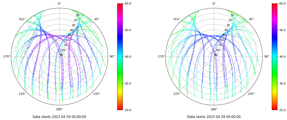
Skyplot for station CEU1. Signal to Noise S1C Data file CEU100ESP_R_2023119.xtr Skyplot for station CEU1. Signal to Noise S2C Data file CEU100ESP_R_2023119.xtr
