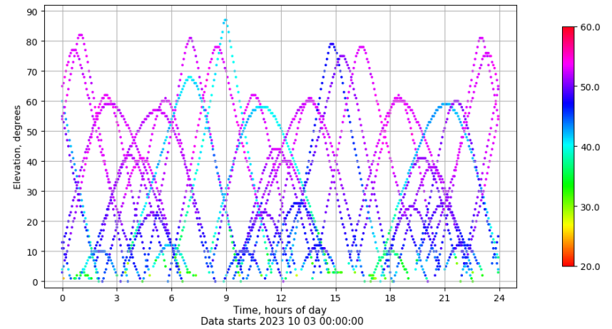
Time-elevation plot for station CBON. Signal to Noise S1C Data file CBON00ESP_R_2023276.xtr
