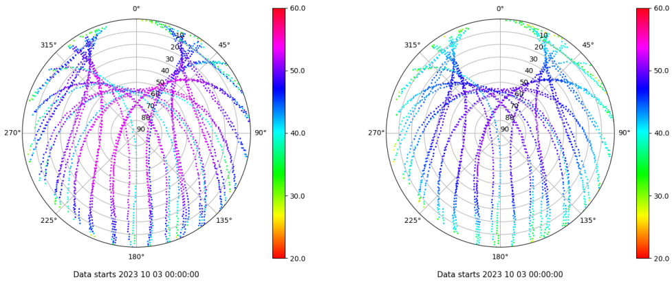
Skyplot for station CBON. Signal to Noise S1C Data file CBON00ESP_R_2023276.xtr Skyplot for station CBON. Signal to Noise S2P Data file CBON00ESP_R_2023276.xtr
