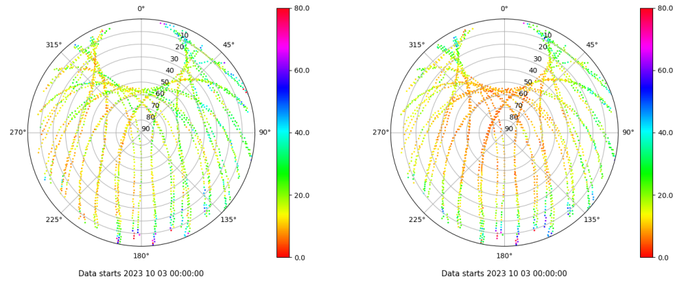
Skyplot for station CBON. Parameter M1C Data file CBON00ESP_R_2023276.xtr Skyplot for station CBON. Parameter M2P Data file CBON00ESP_R_2023276.xtr
