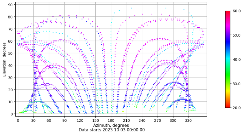
Azimuth-elevation plot for station CBON. Signal to Noise S1C Data file CBON00ESP_R_2023276.xtr
