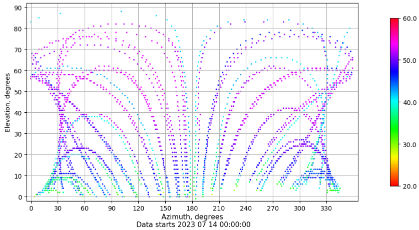
Azimuth-elevation plot for station CBON. Signal to Noise S1C Data file CBON00ESP_R_2023195.xtr
