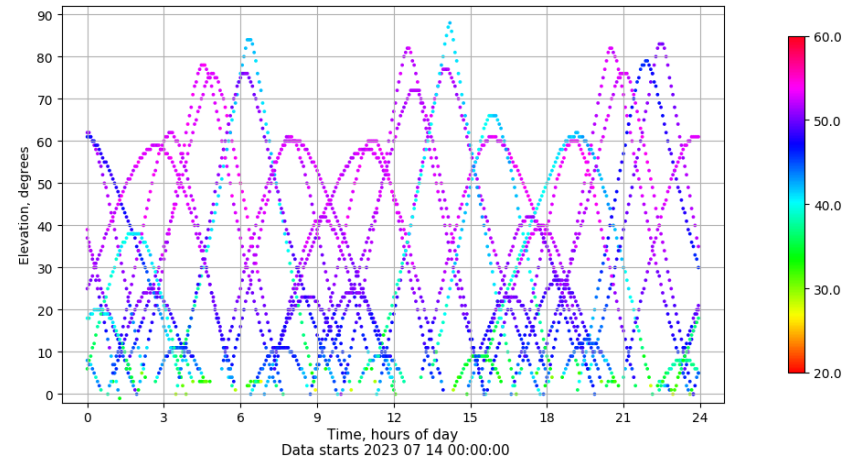
Time-elevation plot for station CBON. Signal to Noise S1C Data file CBON00ESP_R_2023195.xtr
