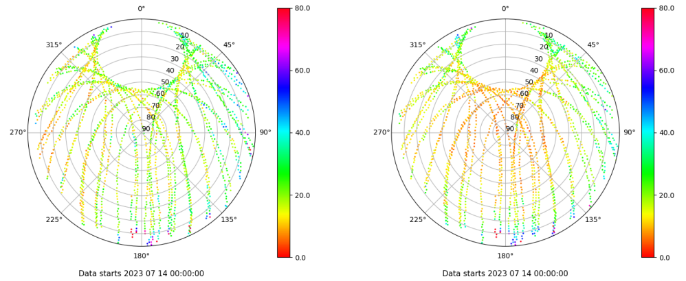
Skyplot for station CBON. Parameter M1C Data file CBON00ESP_R_2023195.xtr Skyplot for station CBON. Parameter M2P Data file CBON00ESP_R_2023195.xtr
