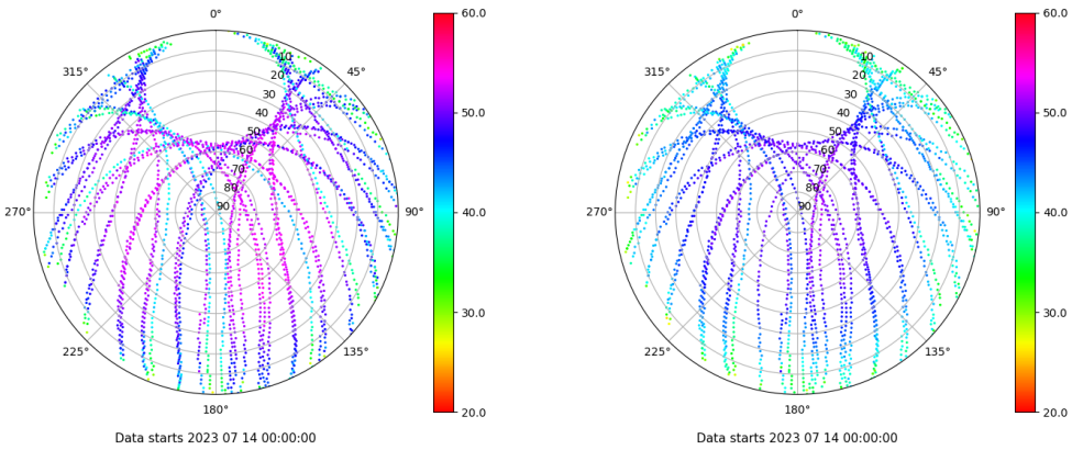
Skyplot for station CBON. Signal to Noise S1C Data file CBON00ESP_R_2023195.xtr Skyplot for station CBON. Signal to Noise S2P Data file CBON00ESP_R_2023195.xtr
