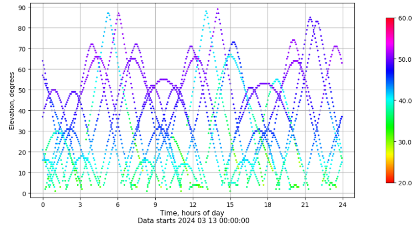
Time-elevation plot for station CAZA. Signal to Noise S1C Data file CAZA00ESP_R_2024073.xtr
