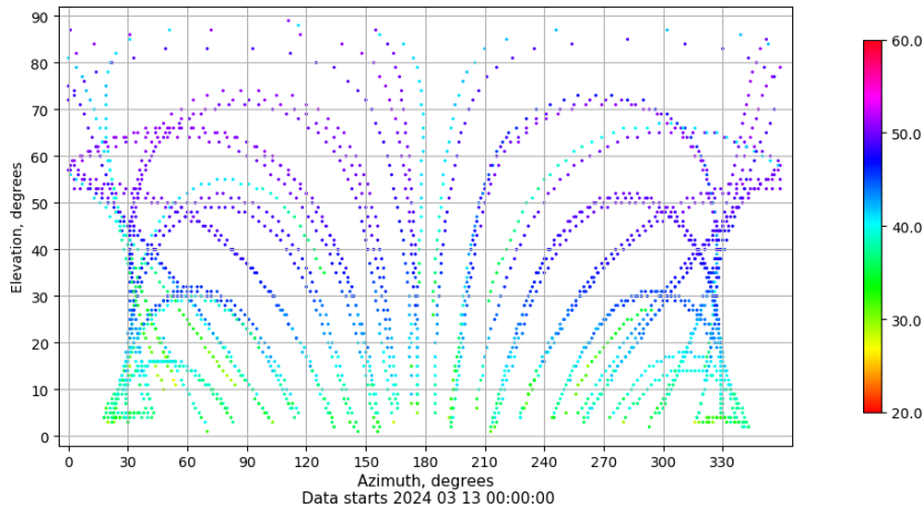
Azimuth-elevation plot for station CAZA. Signal to Noise S1C Data file CAZA00ESP_R_2024073.xtr
