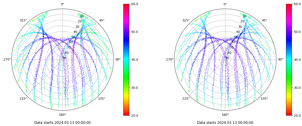
Skyplot for station CAZA. Signal to Noise S1C Data file CAZA00ESP_R_2024073.xtr Skyplot for station CAZA. Signal to Noise S2P Data file CAZA00ESP_R_2024073.xtr
