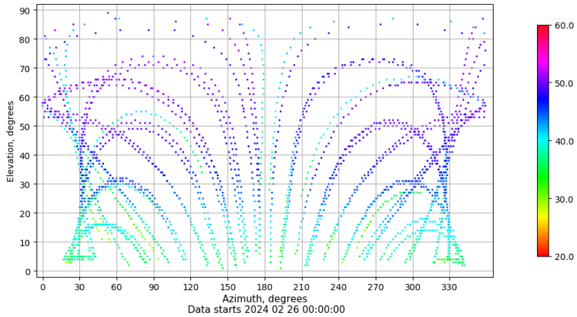
Azimuth-elevation plot for station CAZA. Signal to Noise S1C Data file CAZA00ESP_R_2024057.xtr
