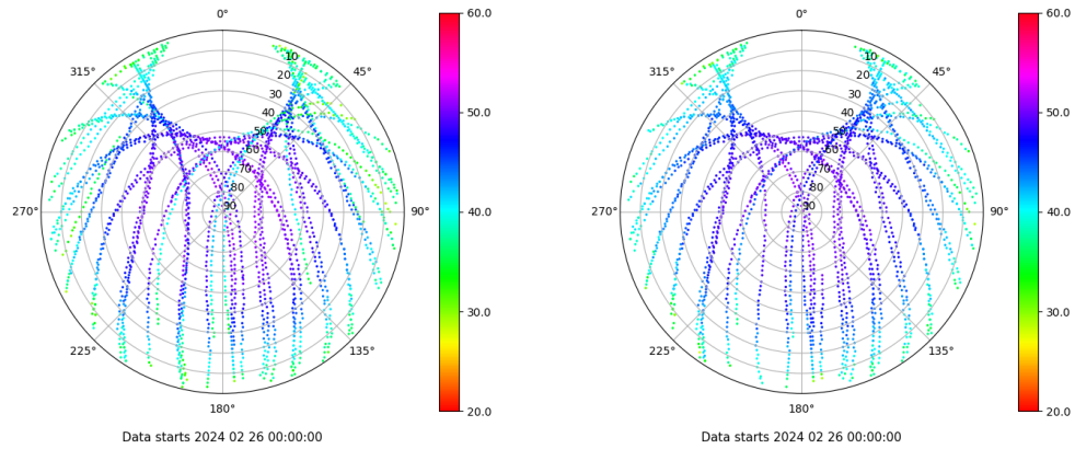
Skyplot for station CAZA. Signal to Noise S1C Data file CAZA00ESP_R_2024057.xtr Skyplot for station CAZA. Signal to Noise S2P Data file CAZA00ESP_R_2024057.xtr
