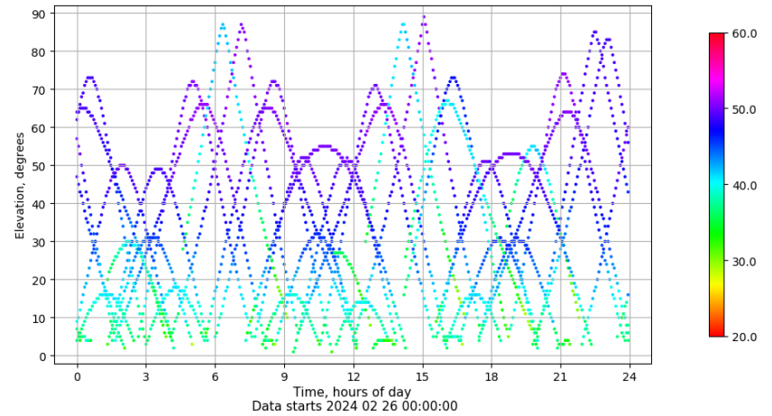
Time-elevation plot for station CAZA. Signal to Noise S1C Data file CAZA00ESP_R_2024057.xtr
