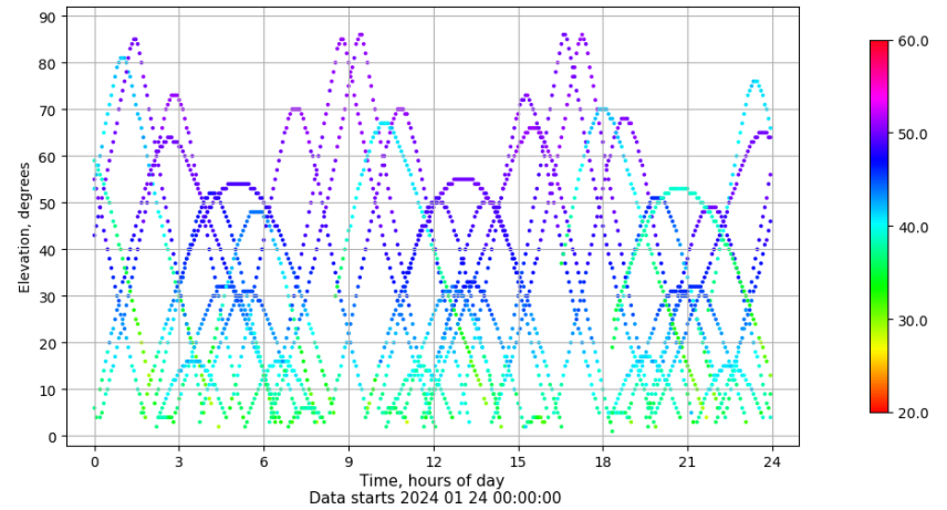
Time-elevation plot for station CAZA. Signal to Noise S1C Data file CAZA00ESP_R_2024024.xtr
