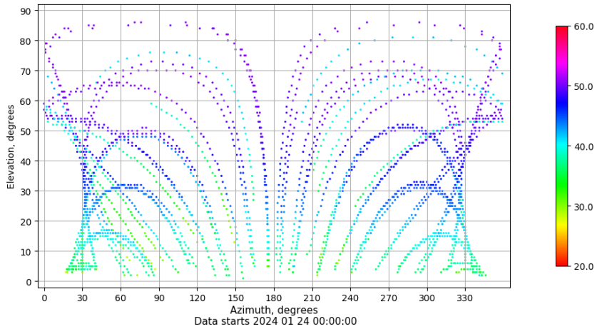
Azimuth-elevation plot for station CAZA. Signal to Noise S1C Data file CAZA00ESP_R_2024024.xtr
