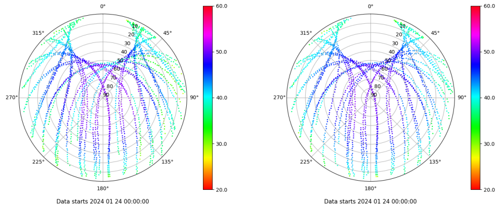
Skyplot for station CAZA. Signal to Noise S1C Data file CAZA00ESP_R_2024024.xtr Skyplot for station CAZA. Signal to Noise S2P Data file CAZA00ESP_R_2024024.xtr
