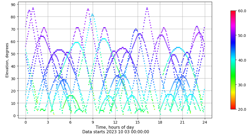
Time-elevation plot for station CAZA. Signal to Noise S1C Data file CAZA00ESP_R_2023276.xtr
