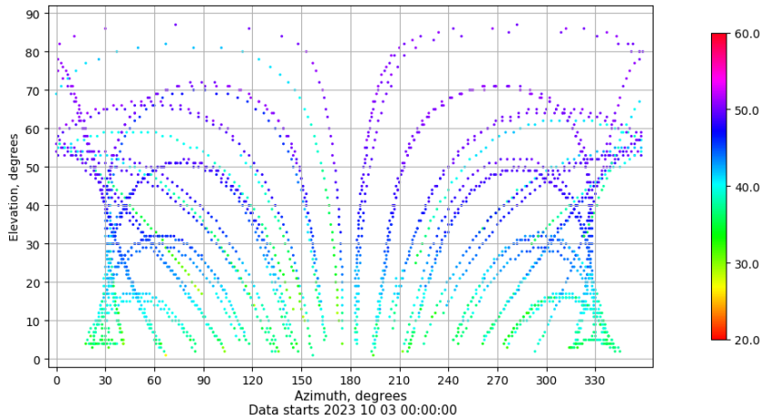
Azimuth-elevation plot for station CAZA. Signal to Noise S1C Data file CAZA00ESP_R_2023276.xtr
