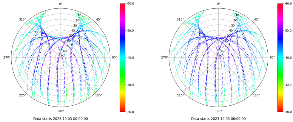
Skyplot for station CAZA. Signal to Noise S1C Data file CAZA00ESP_R_2023276.xtr Skyplot for station CAZA. Signal to Noise S2P Data file CAZA00ESP_R_2023276.xtr
