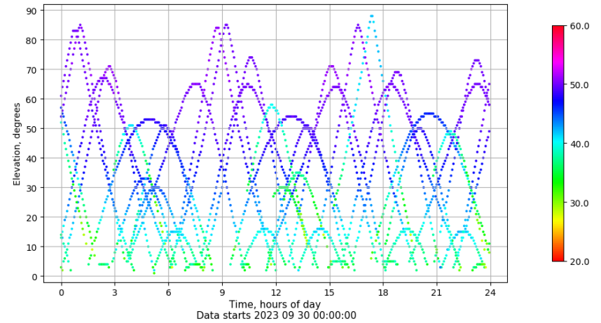
Time-elevation plot for station CAZA. Signal to Noise S1C Data file CAZA00ESP_R_2023273.xtr
