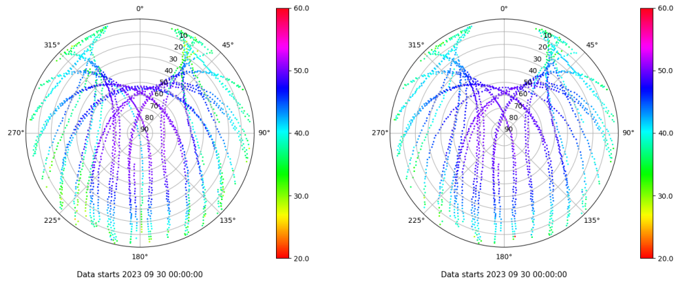
Skyplot for station CAZA. Signal to Noise S1C Data file CAZA00ESP_R_2023273.xtr Skyplot for station CAZA. Signal to Noise S2P Data file CAZA00ESP_R_2023273.xtr
