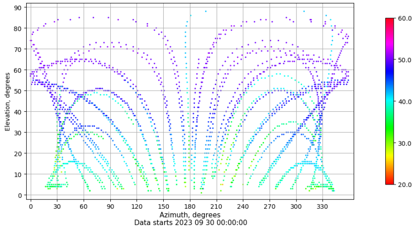
Azimuth-elevation plot for station CAZA. Signal to Noise S1C Data file CAZA00ESP_R_2023273.xtr
