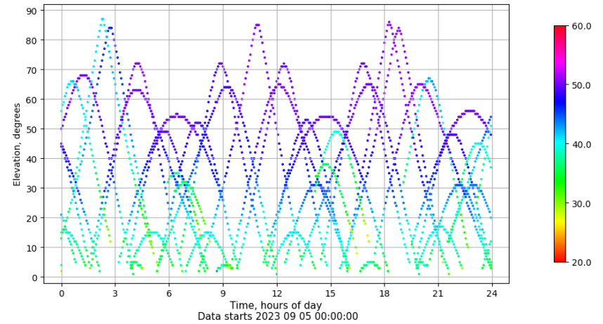
Time-elevation plot for station CAZA. Signal to Noise S1C Data file CAZA00ESP_R_2023248.xtr
