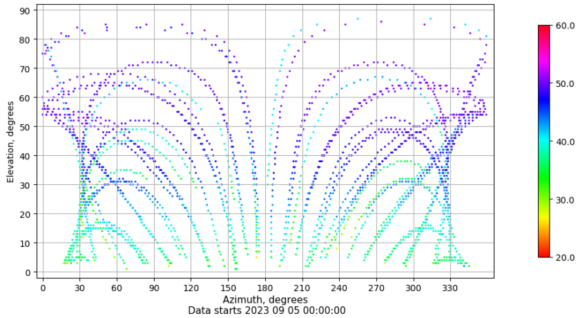
Azimuth-elevation plot for station CAZA. Signal to Noise S1C Data file CAZA00ESP_R_2023248.xtr
