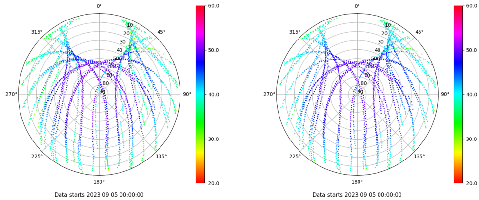
Skyplot for station CAZA. Signal to Noise S1C Data file CAZA00ESP_R_2023248.xtr Skyplot for station CAZA. Signal to Noise S2P Data file CAZA00ESP_R_2023248.xtr
