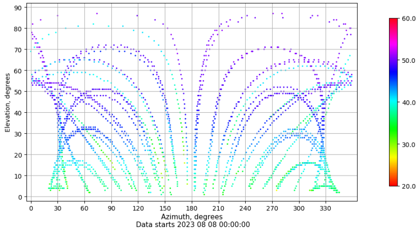
Azimuth-elevation plot for station CAZA. Signal to Noise S1C Data file CAZA00ESP_R_2023220.xtr
