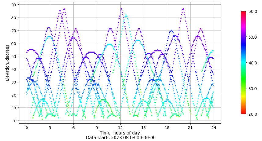
Time-elevation plot for station CAZA. Signal to Noise S1C Data file CAZA00ESP_R_2023220.xtr
