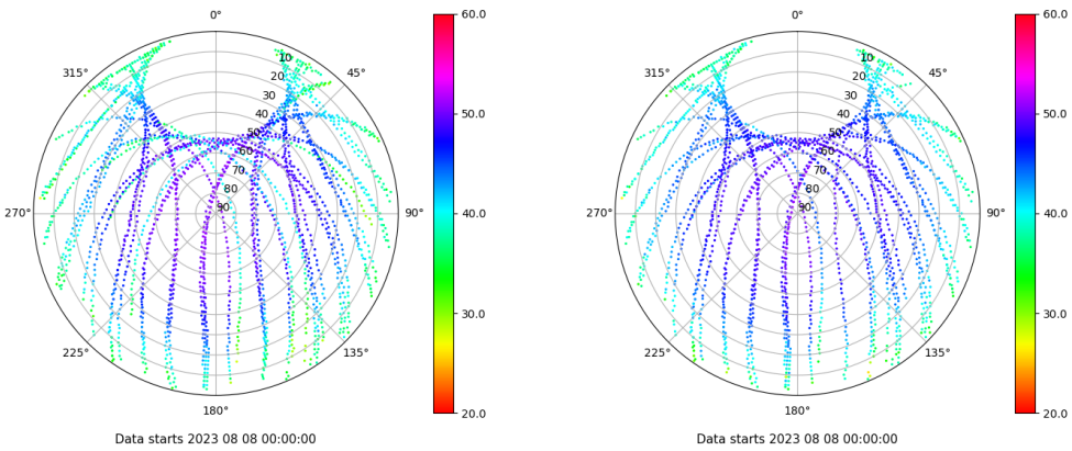
Skyplot for station CAZA. Signal to Noise S1C Data file CAZA00ESP_R_2023220.xtr Skyplot for station CAZA. Signal to Noise S2P Data file CAZA00ESP_R_2023220.xtr
