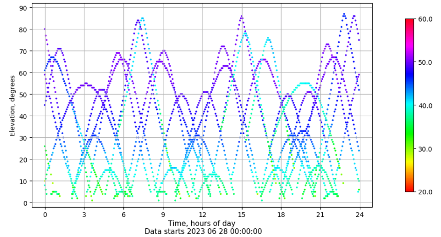
Time-elevation plot for station CAZA. Signal to Noise S1C Data file CAZA00ESP_R_2023179.xtr
