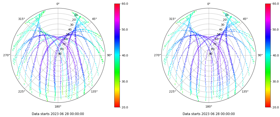
Skyplot for station CAZA. Signal to Noise S1C Data file CAZA00ESP_R_2023179.xtr Skyplot for station CAZA. Signal to Noise S2P Data file CAZA00ESP_R_2023179.xtr
