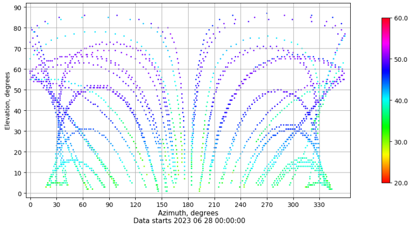
Azimuth-elevation plot for station CAZA. Signal to Noise S1C Data file CAZA00ESP_R_2023179.xtr
