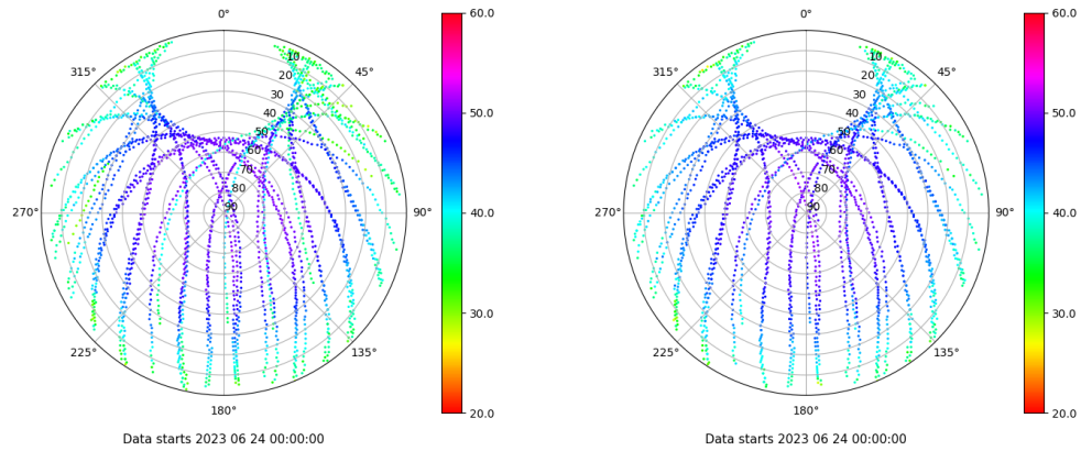
Skyplot for station CAZA. Signal to Noise S1C Data file CAZA00ESP_R_2023175.xtr Skyplot for station CAZA. Signal to Noise S2P Data file CAZA00ESP_R_2023175.xtr
