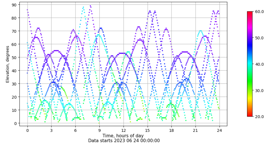
Time-elevation plot for station CAZA. Signal to Noise S1C Data file CAZA00ESP_R_2023175.xtr
