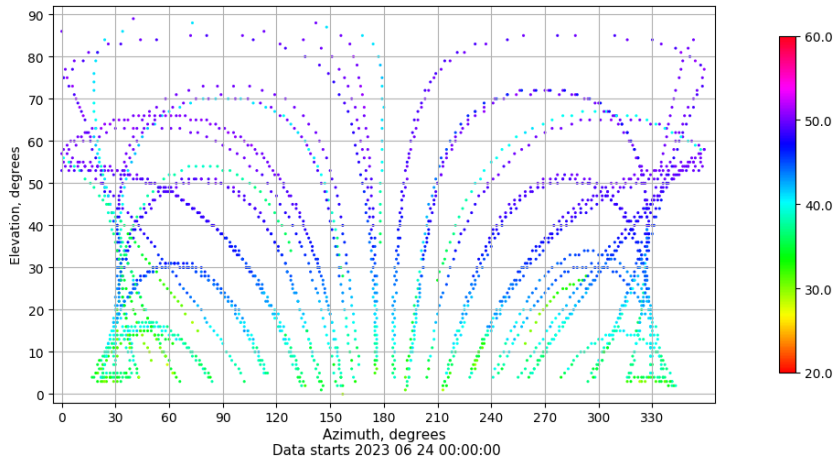
Azimuth-elevation plot for station CAZA. Signal to Noise S1C Data file CAZA00ESP_R_2023175.xtr
