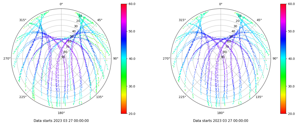
Skyplot for station CAZA. Signal to Noise S1C Data file CAZA00ESP_R_2023086.xtr Skyplot for station CAZA. Signal to Noise S2P Data file CAZA00ESP_R_2023086.xtr
