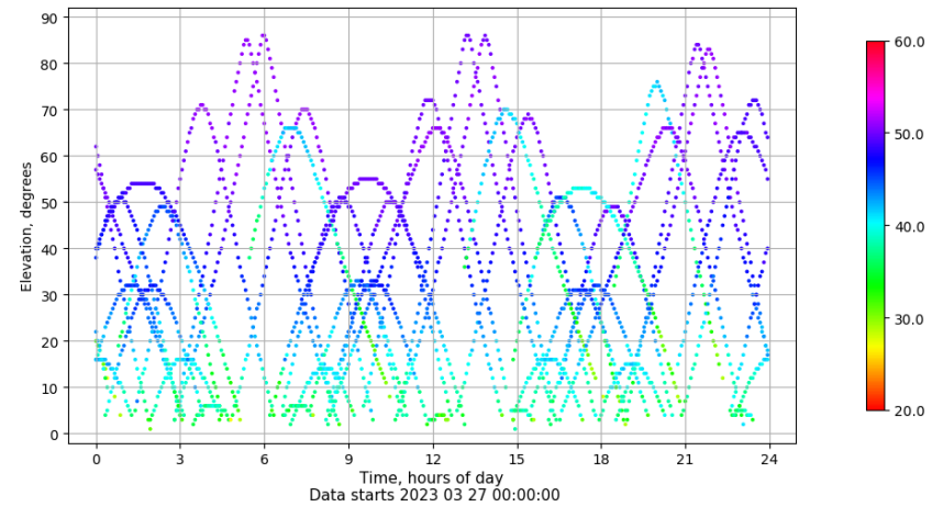
Time-elevation plot for station CAZA. Signal to Noise S1C Data file CAZA00ESP_R_2023086.xtr
