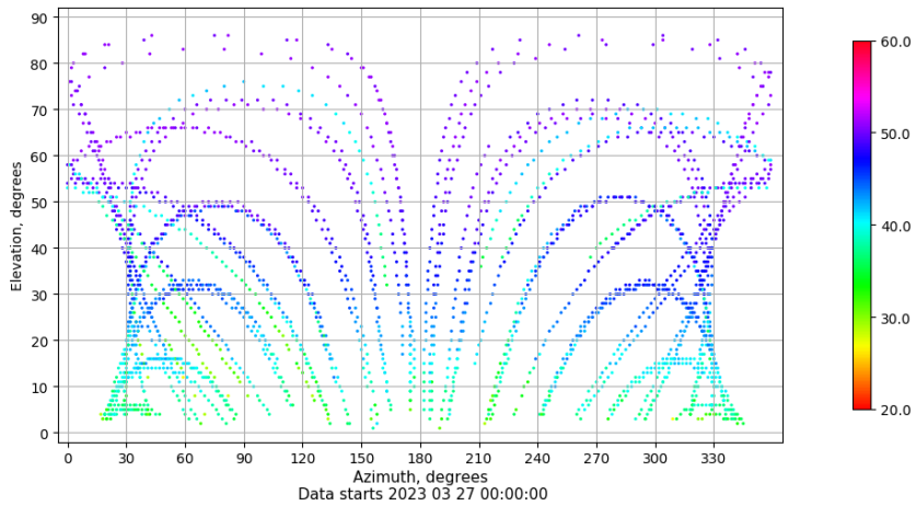
Azimuth-elevation plot for station CAZA. Signal to Noise S1C Data file CAZA00ESP_R_2023086.xtr
