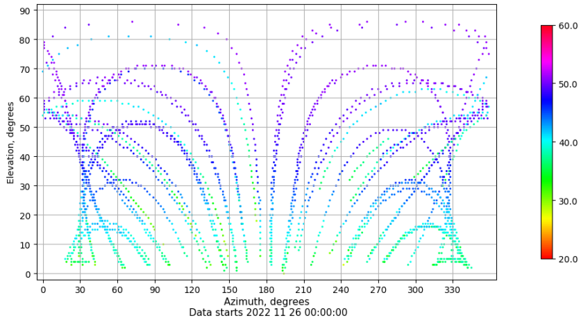
Azimuth-elevation plot for station CAZA. Signal to Noise S1C Data file CAZA00ESP_R_2022330.xtr
