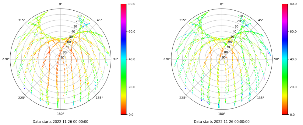
Skyplot for station CAZA. Parameter M1C Data file CAZA00ESP_R_2022330.xtr Skyplot for station CAZA. Parameter M2P Data file CAZA00ESP_R_2022330.xtr
