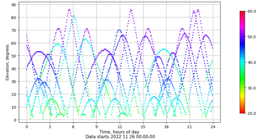
Time-elevation plot for station CAZA. Signal to Noise S1C Data file CAZA00ESP_R_2022330.xtr
