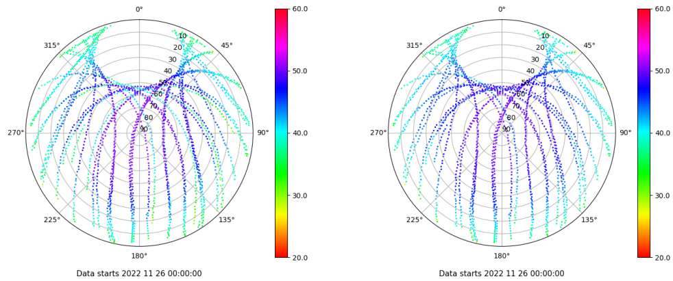
Skyplot for station CAZA. Signal to Noise S1C Data file CAZA00ESP_R_2022330.xtr Skyplot for station CAZA. Signal to Noise S2P Data file CAZA00ESP_R_2022330.xtr
