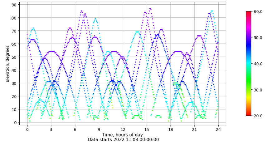
Time-elevation plot for station CAZA. Signal to Noise S1C Data file CAZA00ESP_R_2022312.xtr
