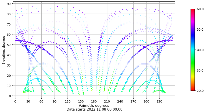
Azimuth-elevation plot for station CAZA. Signal to Noise S1C Data file CAZA00ESP_R_2022312.xtr
