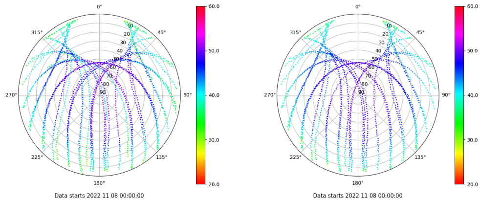
Skyplot for station CAZA. Signal to Noise S1C Data file CAZA00ESP_R_2022312.xtr Skyplot for station CAZA. Signal to Noise S2P Data file CAZA00ESP_R_2022312.xtr
