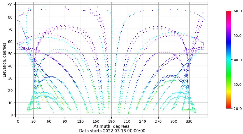
Azimuth-elevation plot for station CAZA. Signal to Noise S1C Data file CAZA00ESP_R_2022077.xtr
