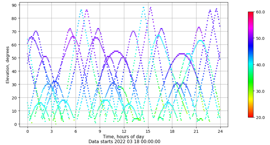
Time-elevation plot for station CAZA. Signal to Noise S1C Data file CAZA00ESP_R_2022077.xtr
