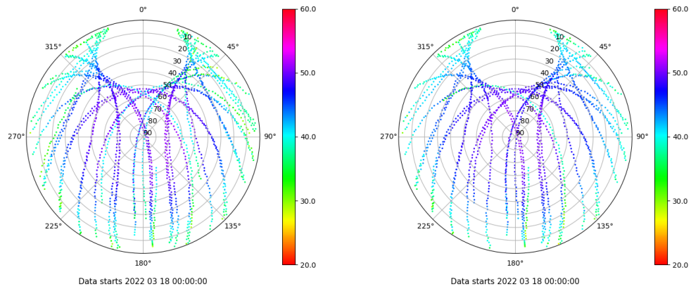
Skyplot for station CAZA. Signal to Noise S1C Data file CAZA00ESP_R_2022077.xtr Skyplot for station CAZA. Signal to Noise S2P Data file CAZA00ESP_R_2022077.xtr
