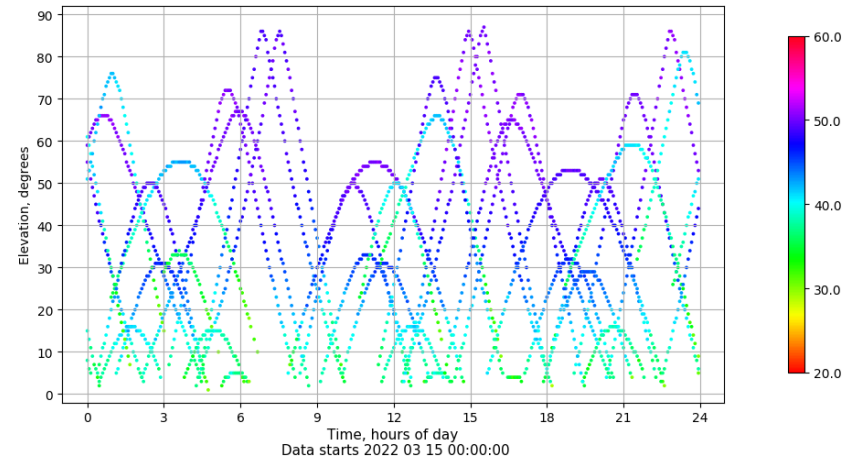
Time-elevation plot for station CAZA. Signal to Noise S1C Data file CAZA00ESP_R_2022074.xtr
