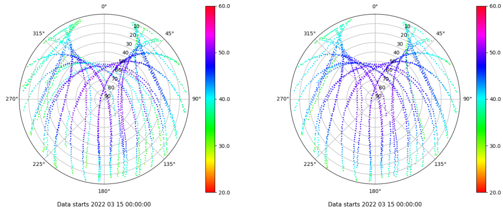
Skyplot for station CAZA. Signal to Noise S1C Data file CAZA00ESP_R_2022074.xtr Skyplot for station CAZA. Signal to Noise S2P Data file CAZA00ESP_R_2022074.xtr
