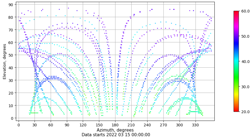
Azimuth-elevation plot for station CAZA. Signal to Noise S1C Data file CAZA00ESP_R_2022074.xtr
