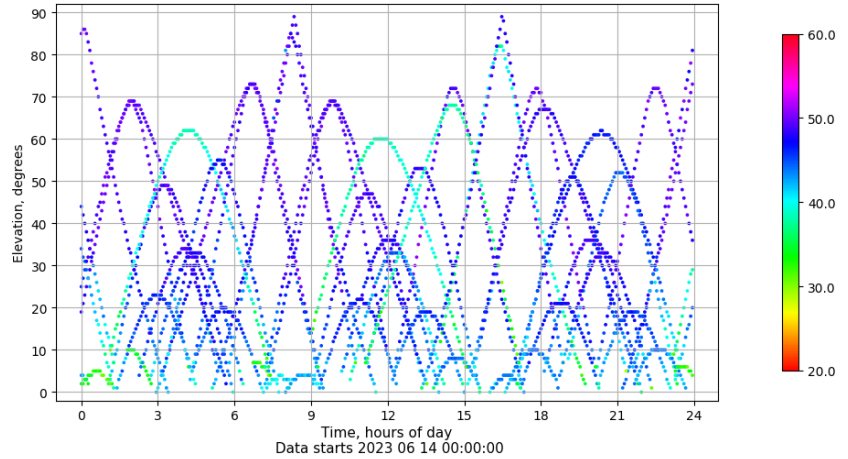
Time-elevation plot for station CANT. Signal to Noise S1C Data file CANT00ESP_R_2023165.xtr
