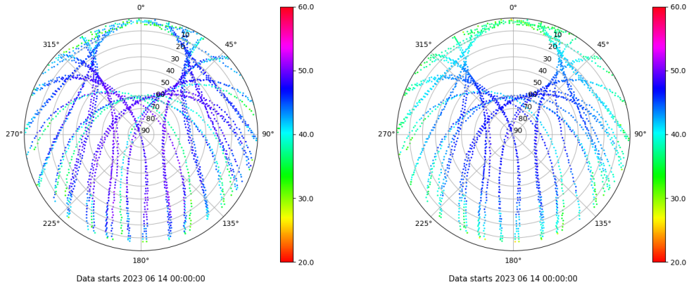
Skyplot for station CANT. Signal to Noise S1C Data file CANT00ESP_R_2023165.xtr Skyplot for station CANT. Signal to Noise S2P Data file CANT00ESP_R_2023165.xtr
