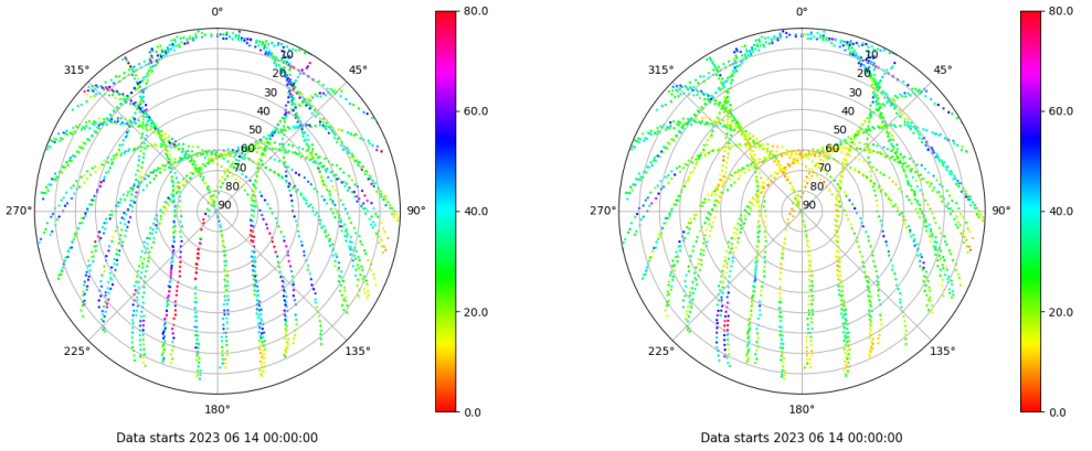
Skyplot for station CANT. Parameter M1C Data file CANT00ESP_R_2023165.xtr Skyplot for station CANT. Parameter M2P Data file CANT00ESP_R_2023165.xtr
