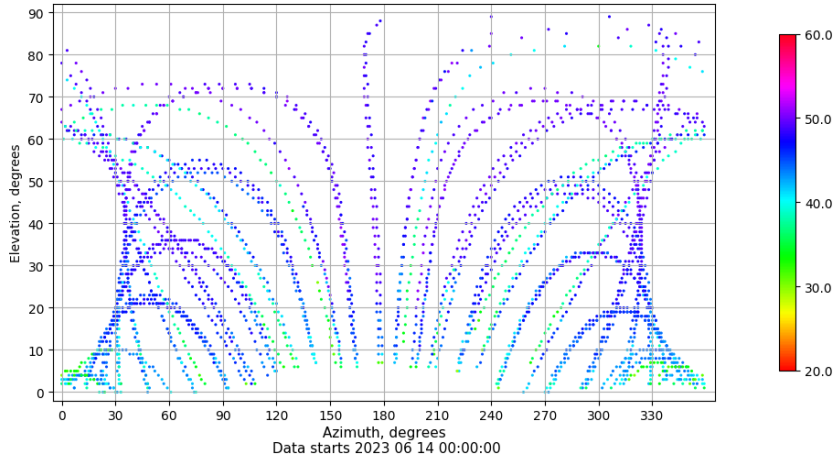
Azimuth-elevation plot for station CANT. Signal to Noise S1C Data file CANT00ESP_R_2023165.xtr
